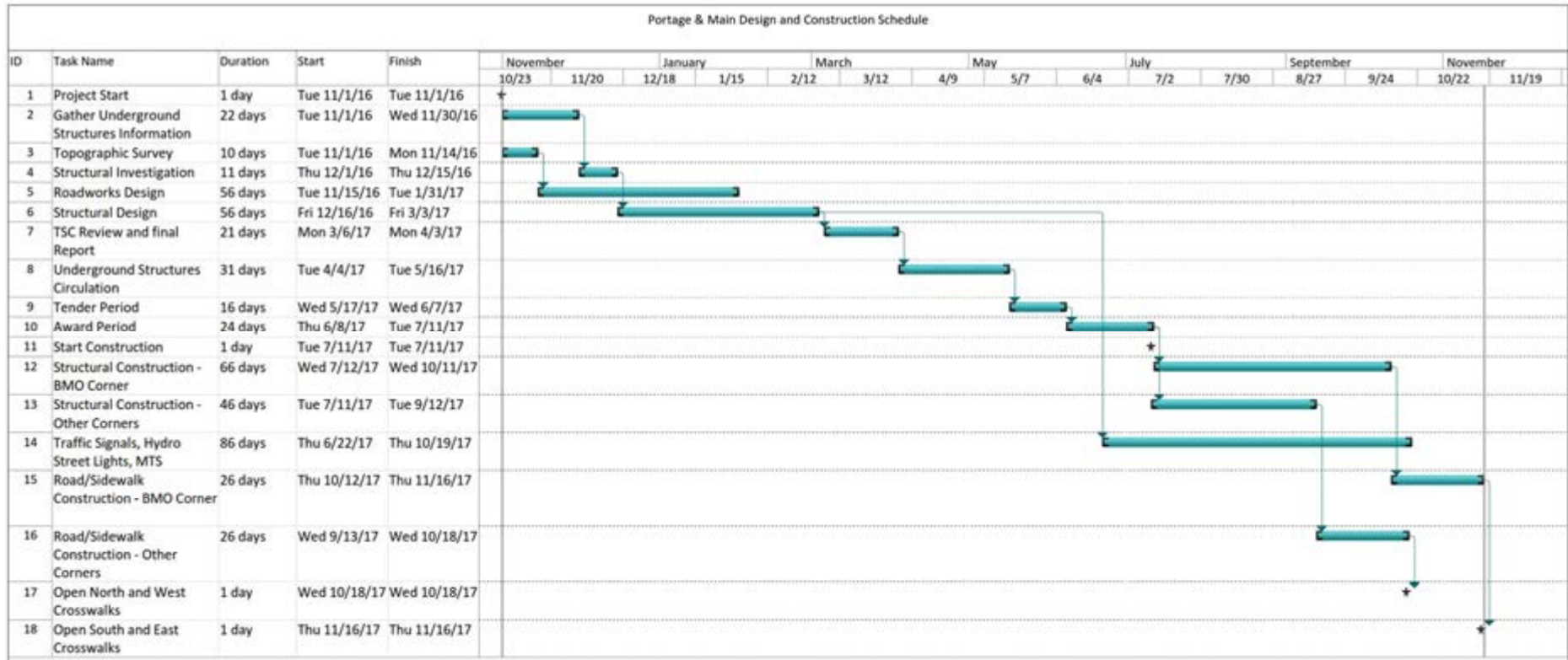
Figure 32 – Design and Construction Schedule
