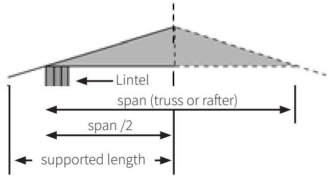
Figure 10 - Supported length of wood lintel
