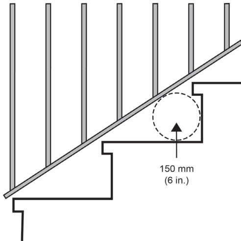
Figure 14: Graspable handrail
