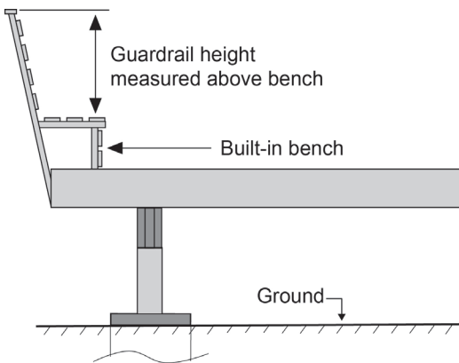
Figure 11: Guardrail and bench
