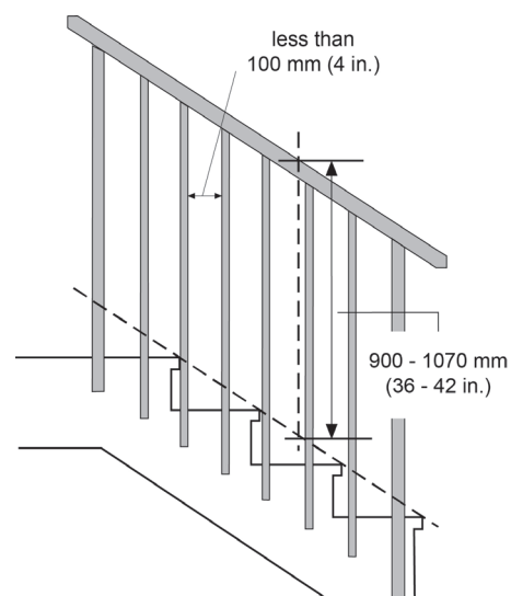
Figure 13: Combine guardrail/handrail
