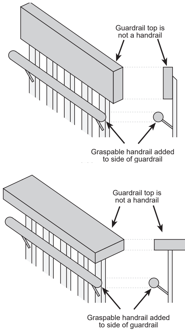
Figure 14: Graspable handrail
