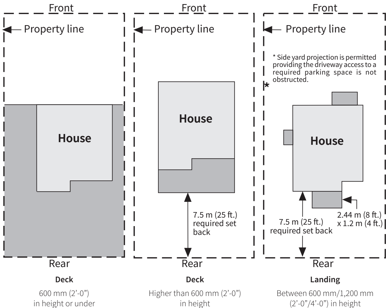
Figure 1: Deck location
