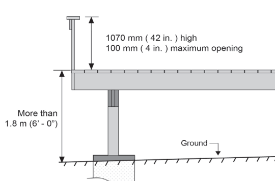
Figure 10: Guardrail height
