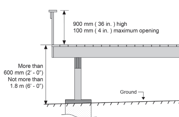
Figure 10: Guardrail height
