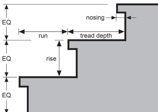
Figure 12: Stair detail
