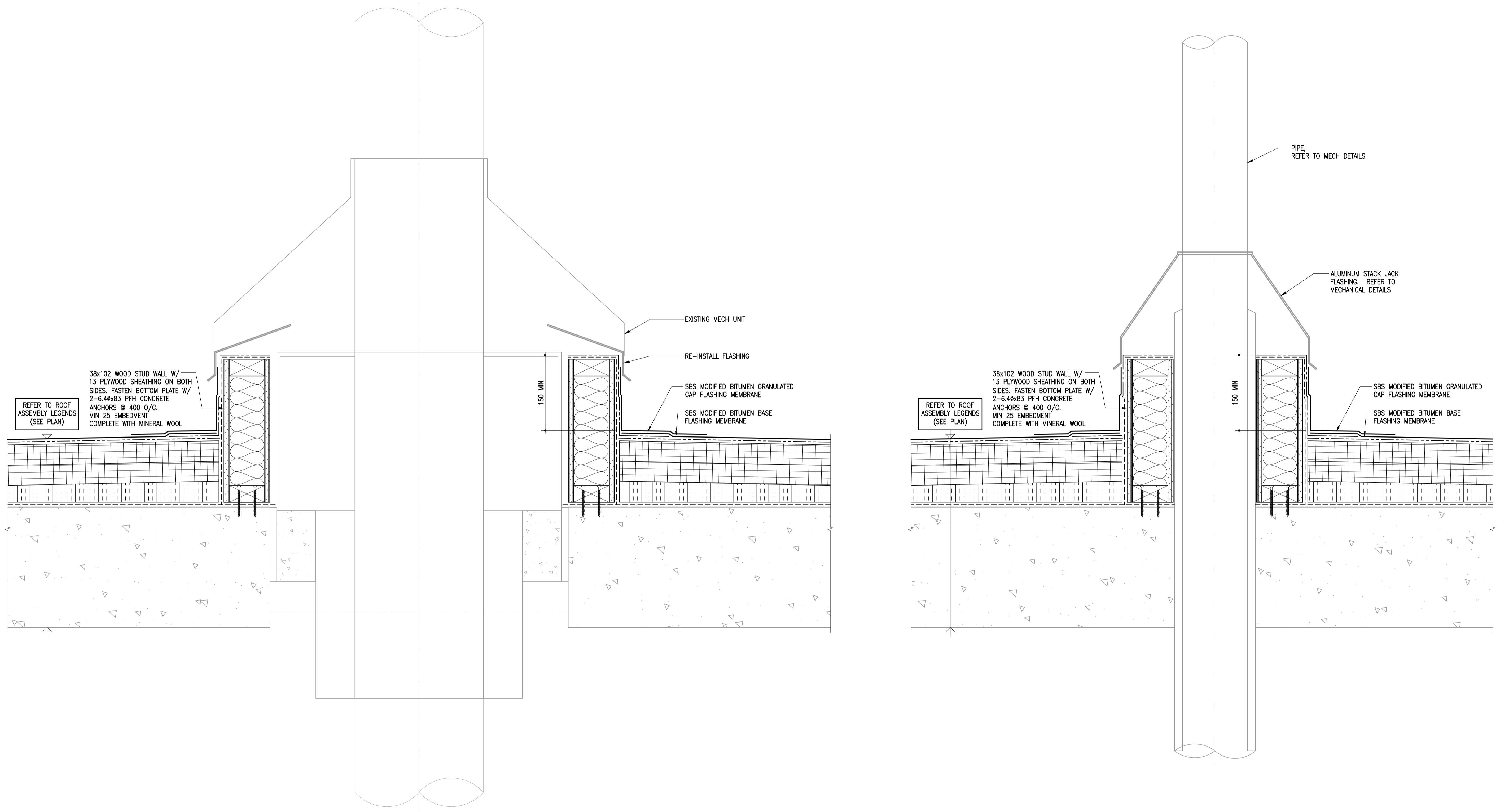
1 GAS FIRED UNIT HEATER AND AIR HANDLING UNIT STACK DETAIL 1-0601B-80076-001 1:5
