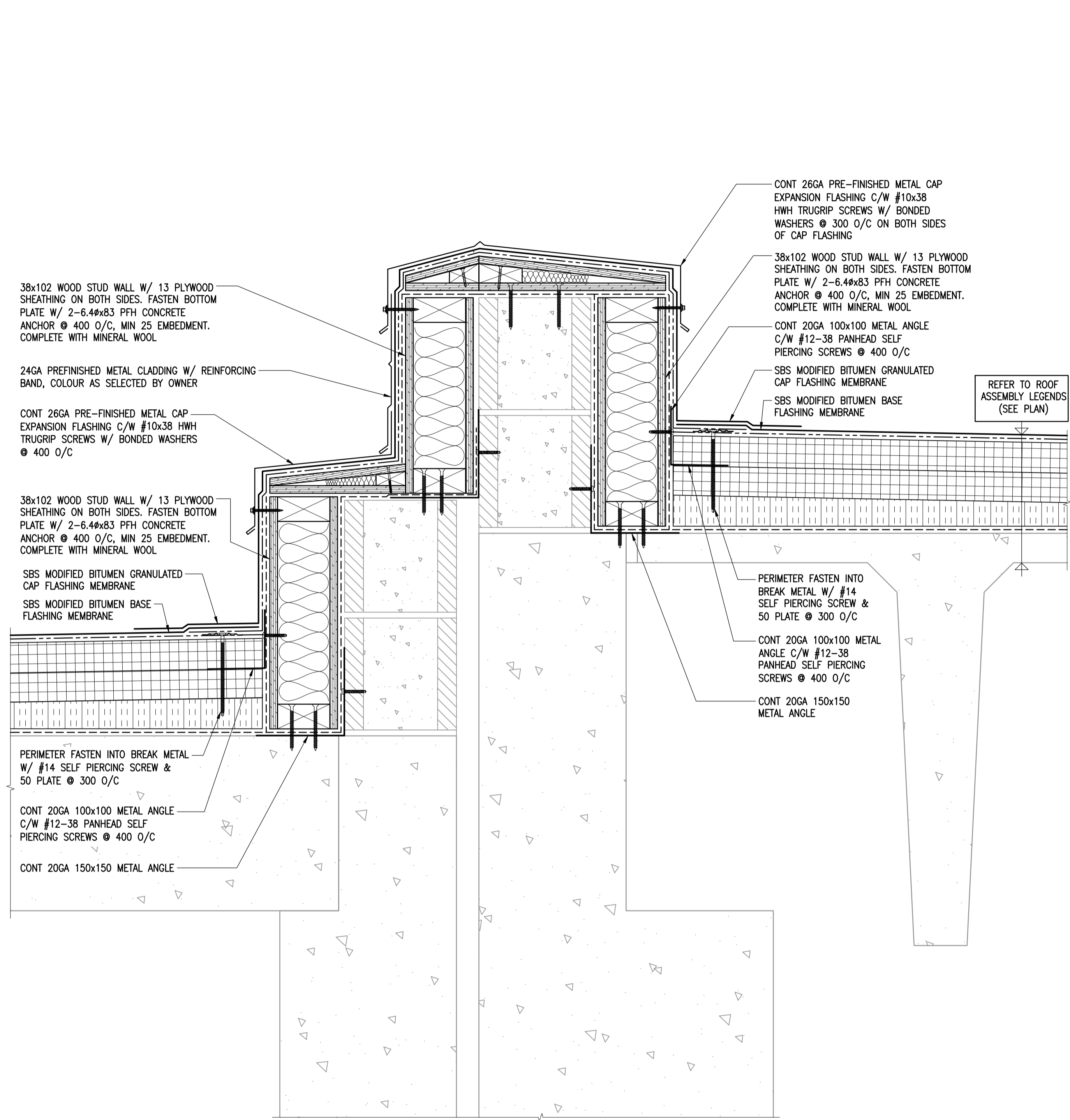
1 ROOF TIE-IN AT PARAPET 1-0601B-80076-04 1:5 (AT VARYING ELEVATIONS)
