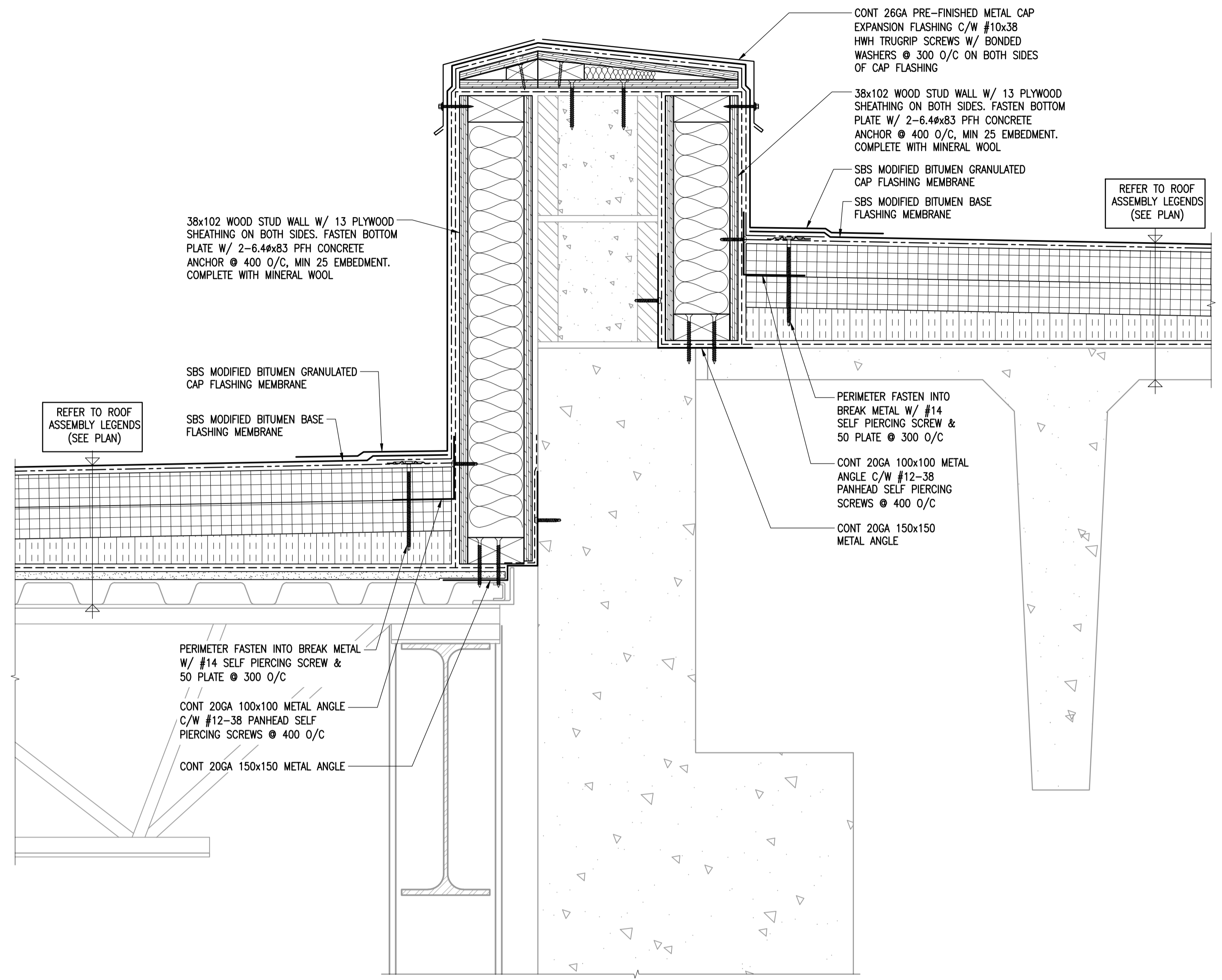
2 ROOF TIE-IN AT PARAPET 1-0601B-80076-04 1:5 (AT VARYING ELEVATIONS)
