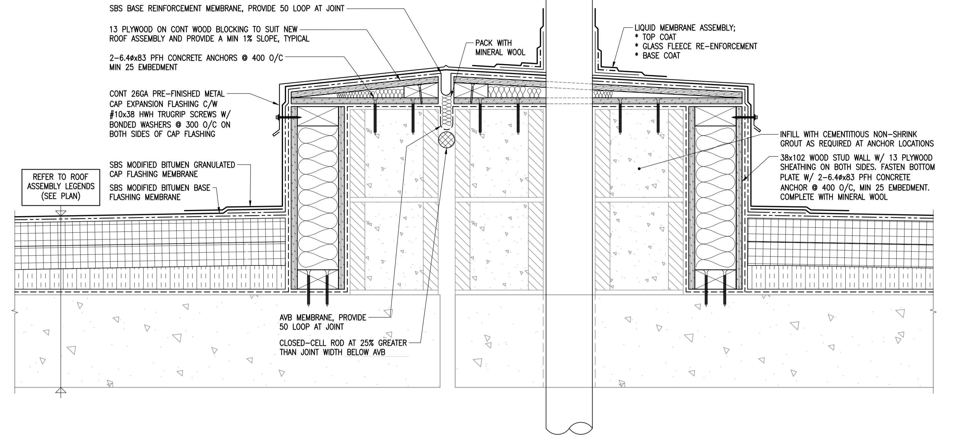
2 LOWER ROOF VENT/EXPANSION JOINT DETAIL 1-0601B-00076-003 1:5
