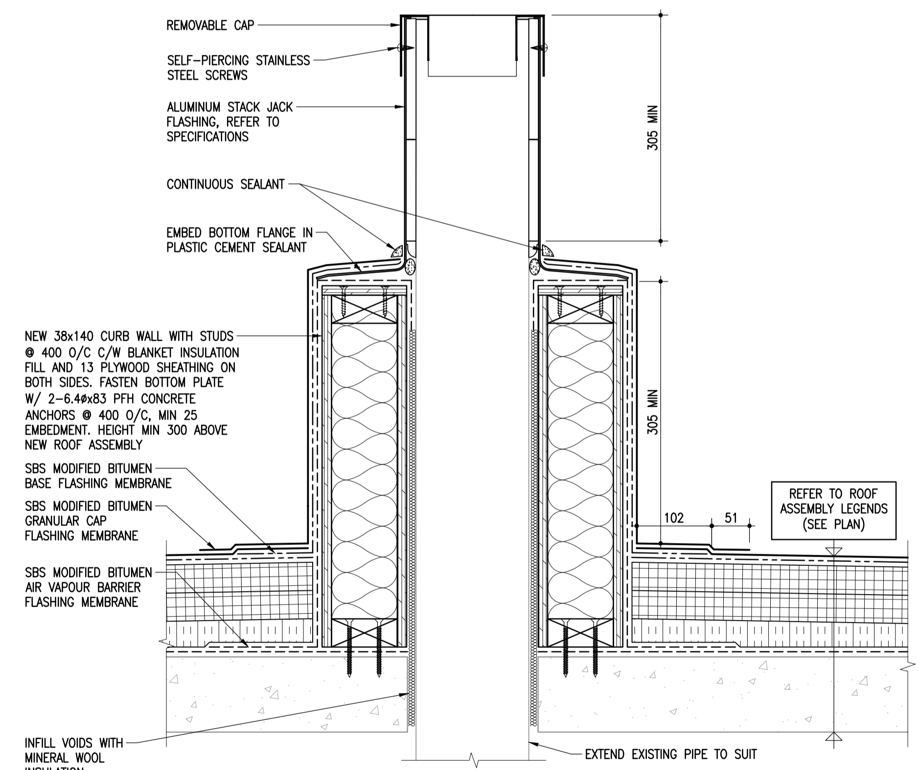
3 TYPICAL VENT/CURB DETAIL 1-0601B-00076-003 1:5
