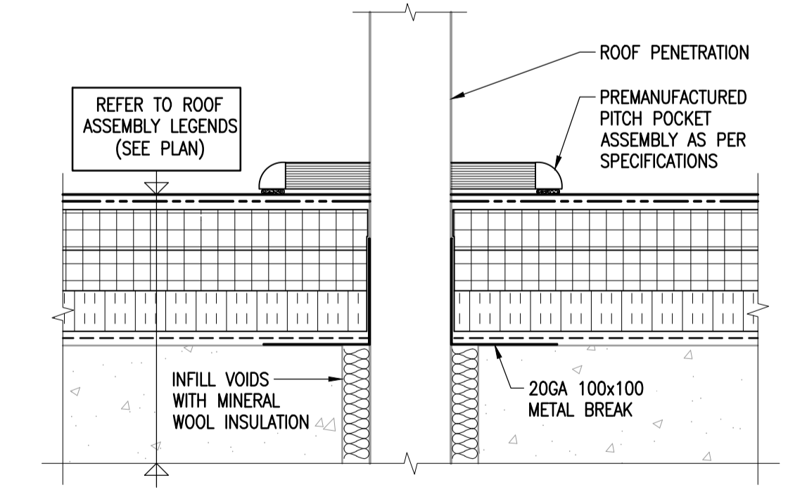
6 TYPICAL PITCH POCKET DETAIL 1-0601B-00076-003 1:5
