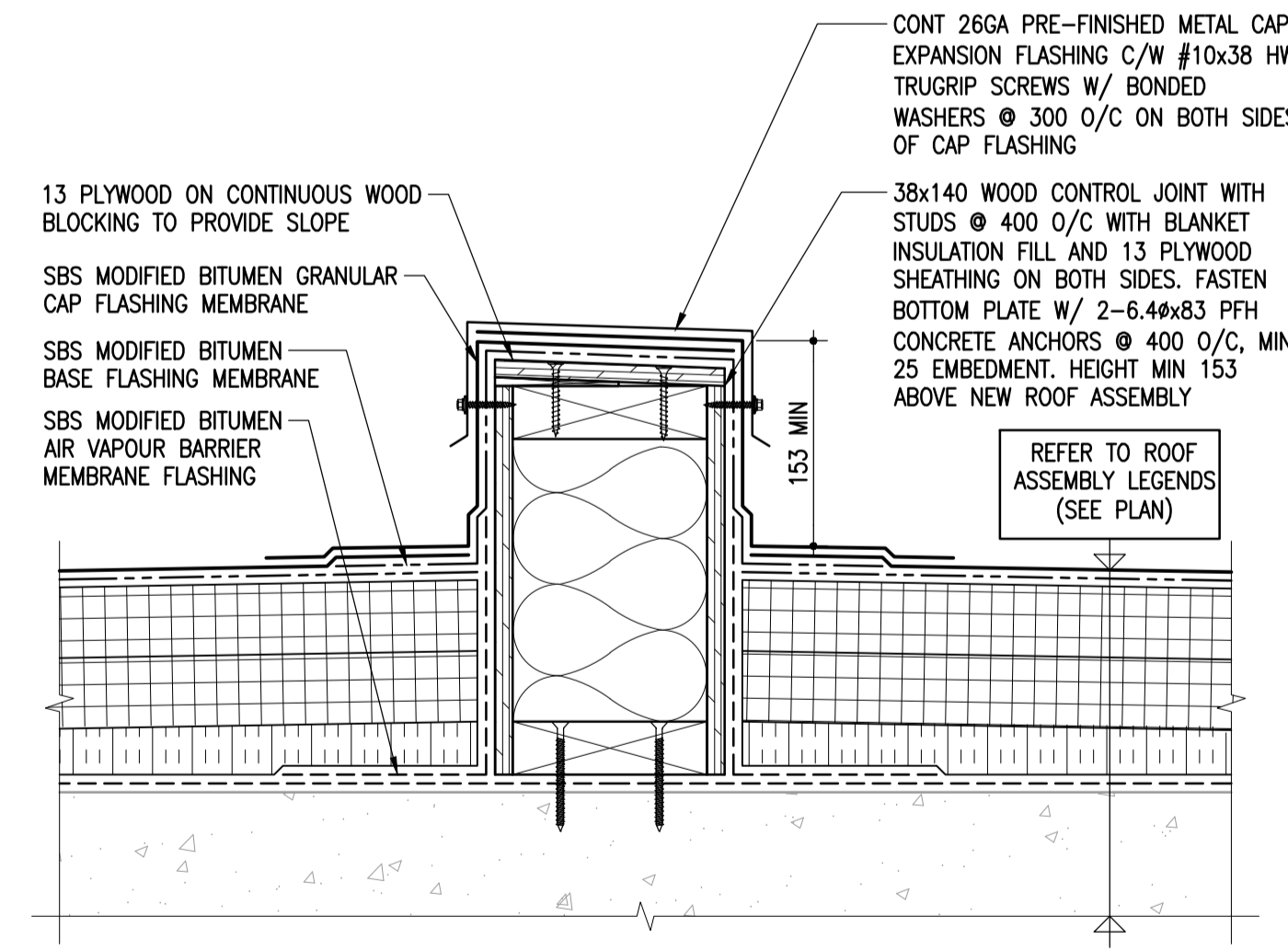
5 TYPICAL CONTROL JOINT DETAIL 1-0601B-00076-003 1:5
