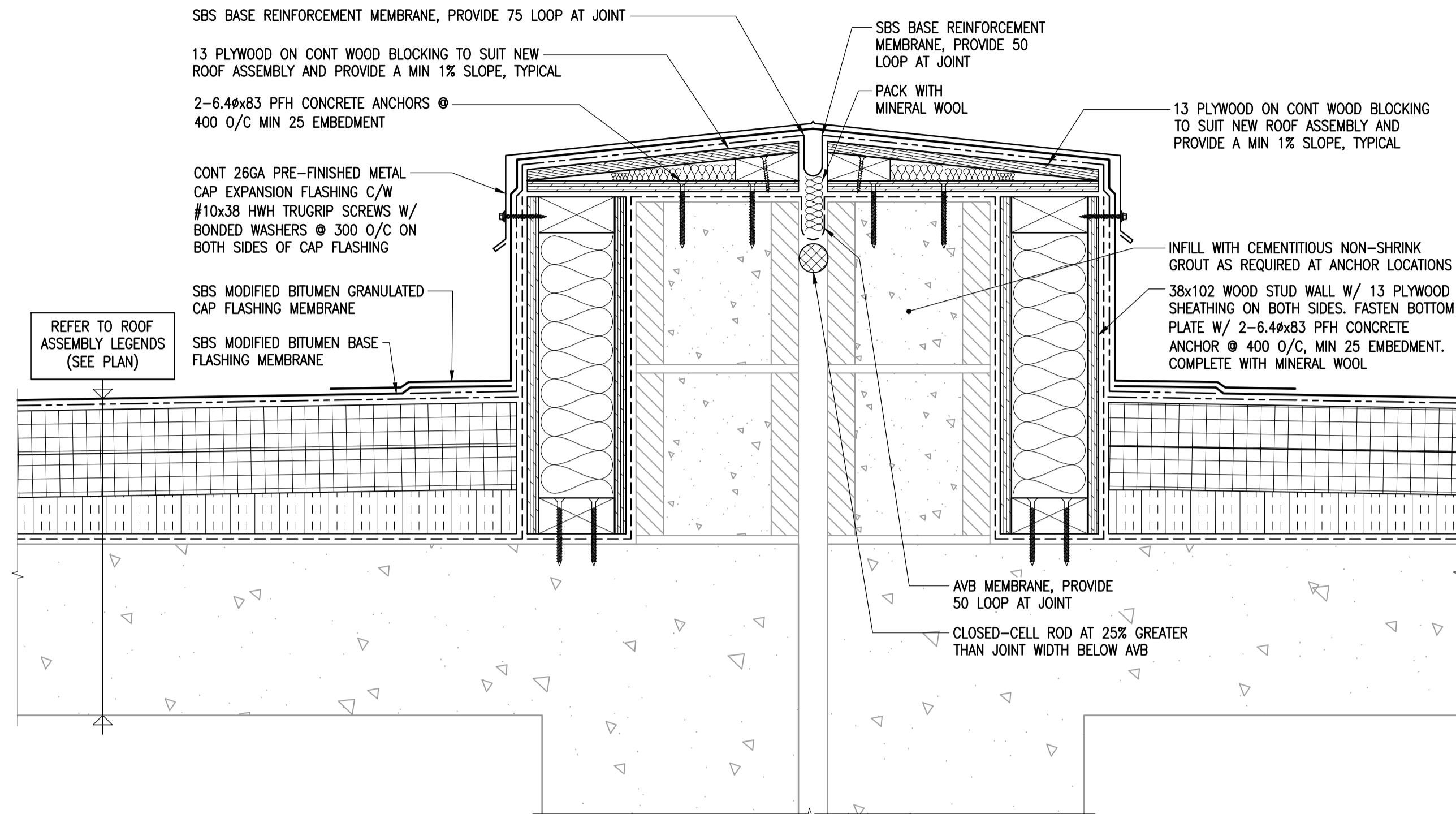
1 ROOF DETAIL AT EXPANSION JOINT 1-0601B-00076-003 1:5
