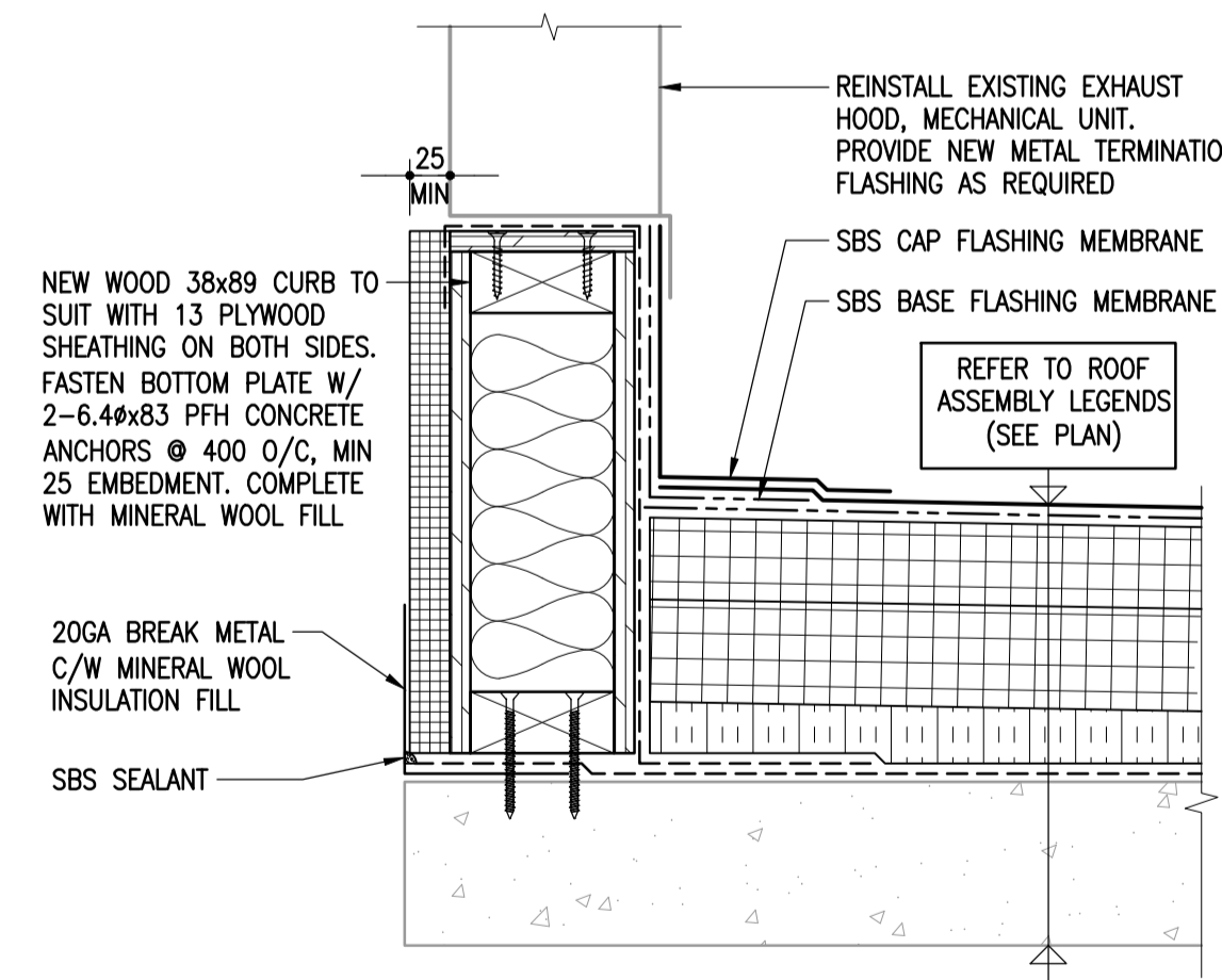
4 TYPICAL CURB DETAIL 1-0601B-00076-003 1:5
