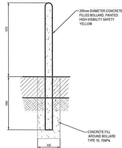
DETAIL 15 TYPICAL BOLLARD NTS
