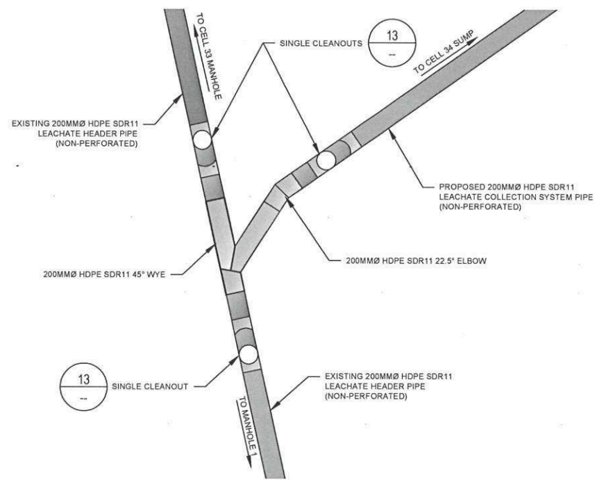
DETAIL 16 LEACHATE EXTRACTION PIPE CONNECTION TO EXISTING LEACHATE HEADER NTS C3001
