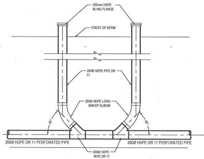
DETAIL 14 SOUTH & WEST DOUBLE CLEAN-OUT RISERS NTS C3001
