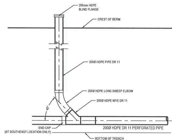
DETAIL 13 SINGLE CLEAN-OUT RISER NTS C3001
