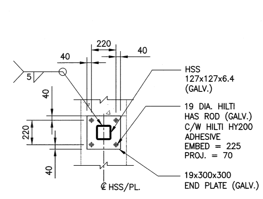
DETAIL 3 1-0650M-S0005 SCALE: 1:20
