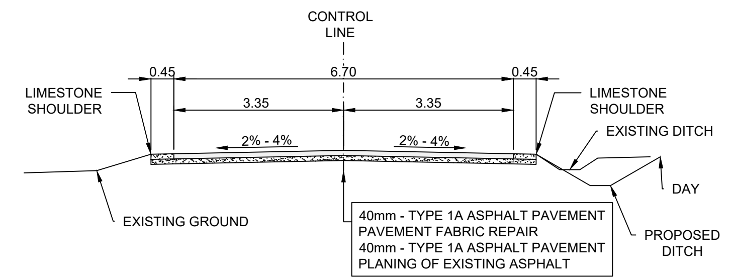
ST VITAL PARK ROAD - MILL & FILL AND ASPHALT DITCH REMOVAL CROSS SECTION (STA: 7+35 - 11+43) N.T.S.
