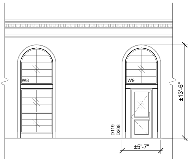
INTERIOR ELEVATION 1':1/8"
