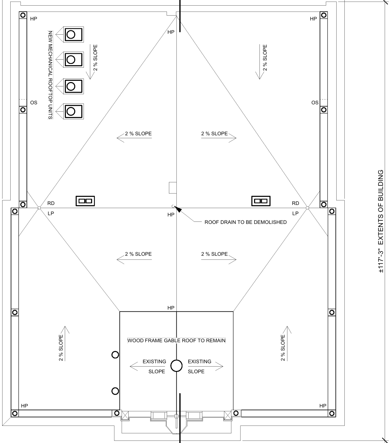
ROOF PLAN 1":1/16" N
