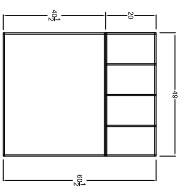
Window W12 Qty = 1 West - Womens Washroom
