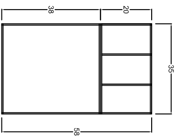
Window W3 Qty = 2 East - Mens Washroom
