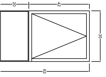
Window W9 Qty = 2 North - Pro Shop
