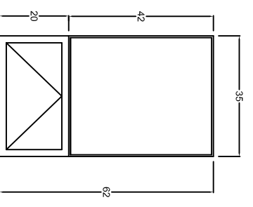
Window W10 Qty = 1 North - Pro Shop
