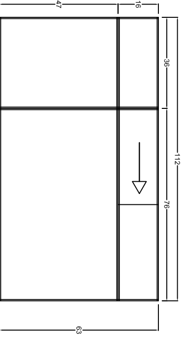
Window W4 Qty = 1 Sunroom - South
