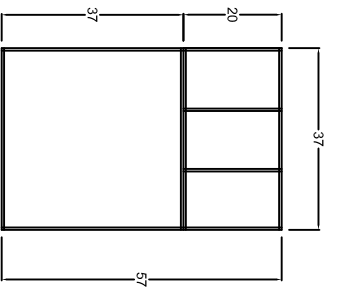
Window W8 Qty = 2 East - Kitchen
