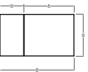
Window W11 Qty = 1 North - Womens Washroom
