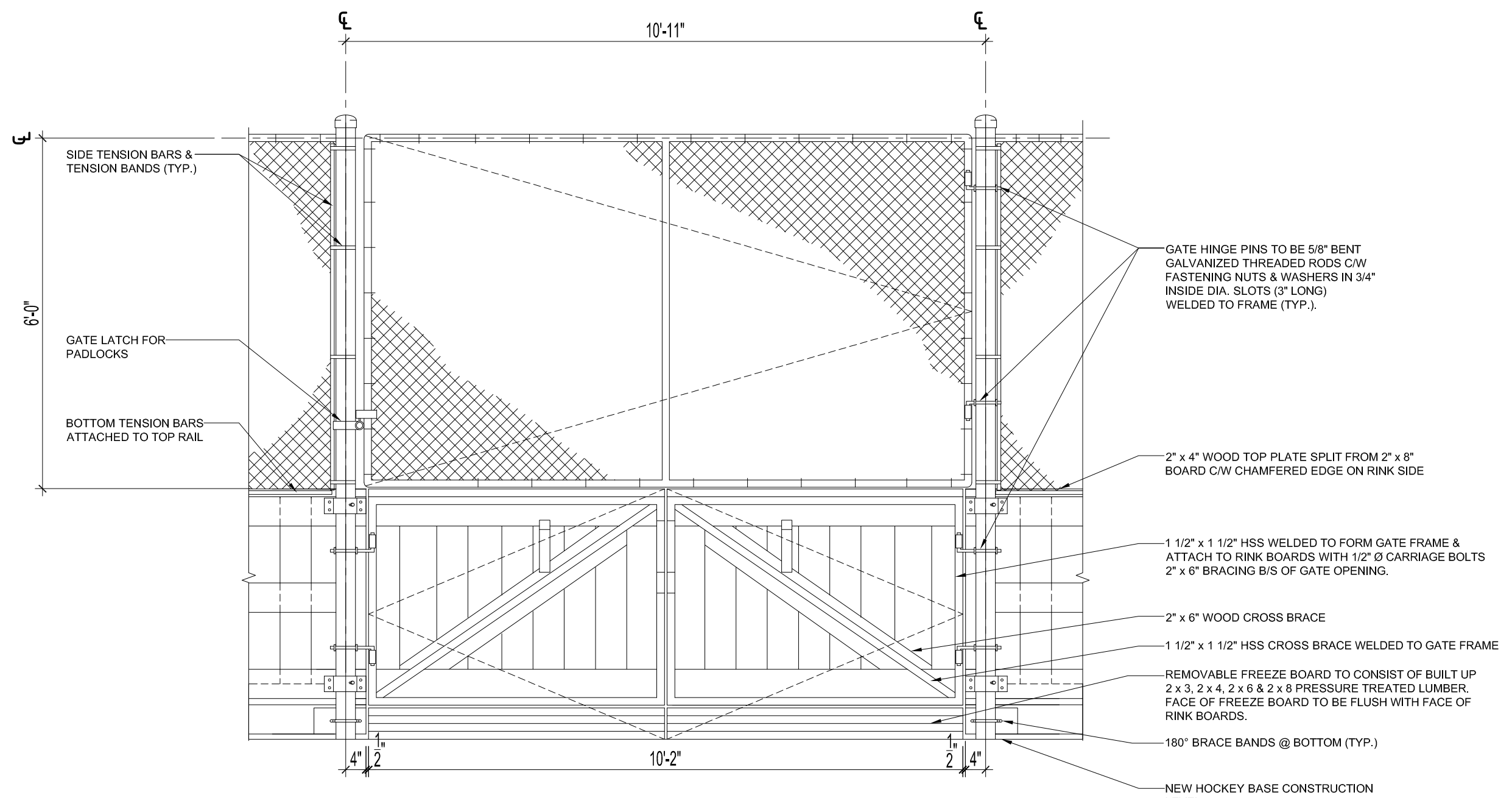
VEHICLE GATE ELEVATION -SWINGING GATE SCALE: 1/2" = 1'-0"
