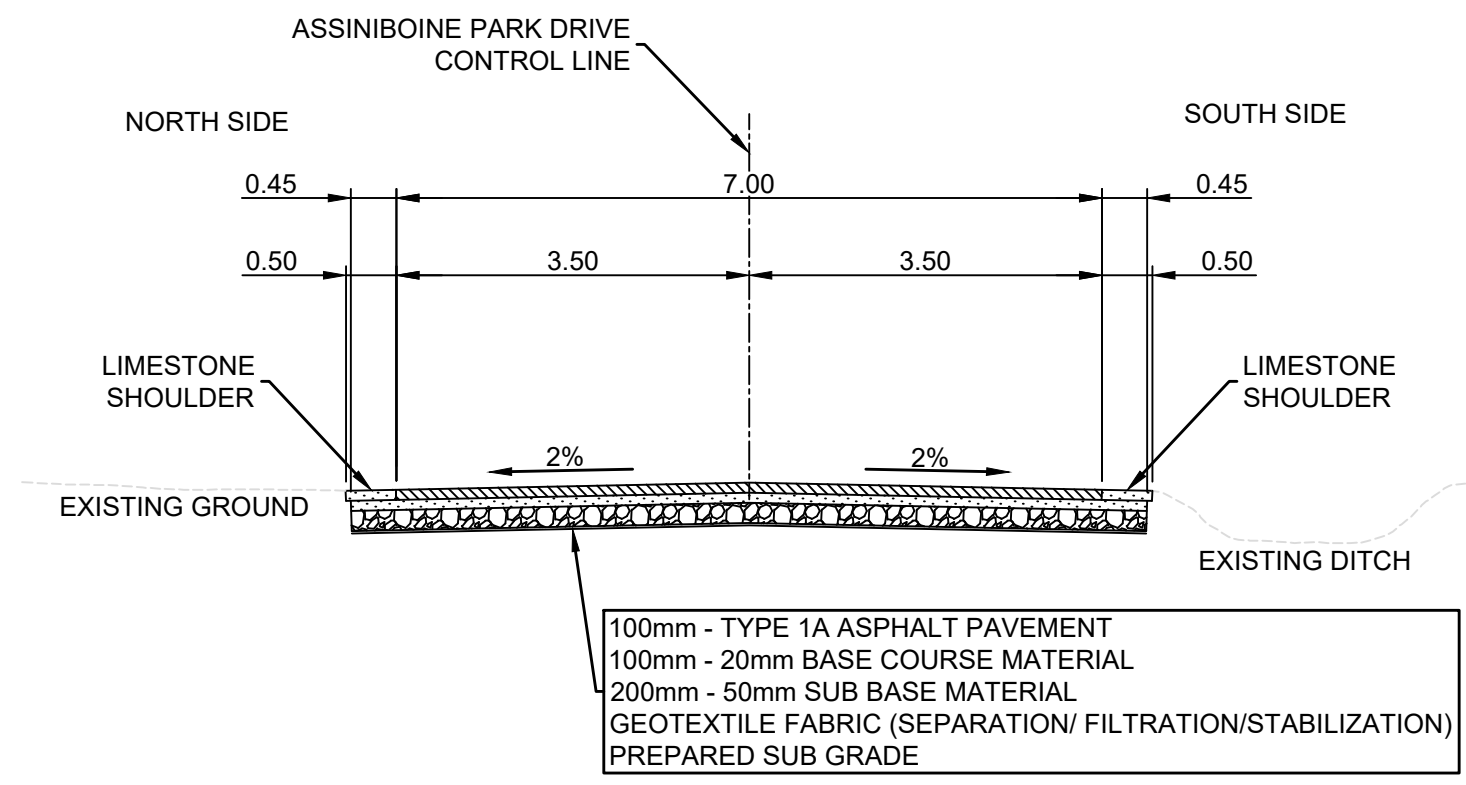
ASSINIBOINE PARK DRIVE - ASPHALT RECONSTRUCTION CROSS SECTION (TYPICAL)
