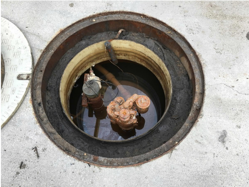
Photograph 3. Damaged Tank Turbine and Sensor ↑
