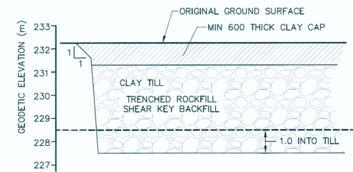
TRENCHED ROCKFILL SHEAR KEY SCALE: NTS
