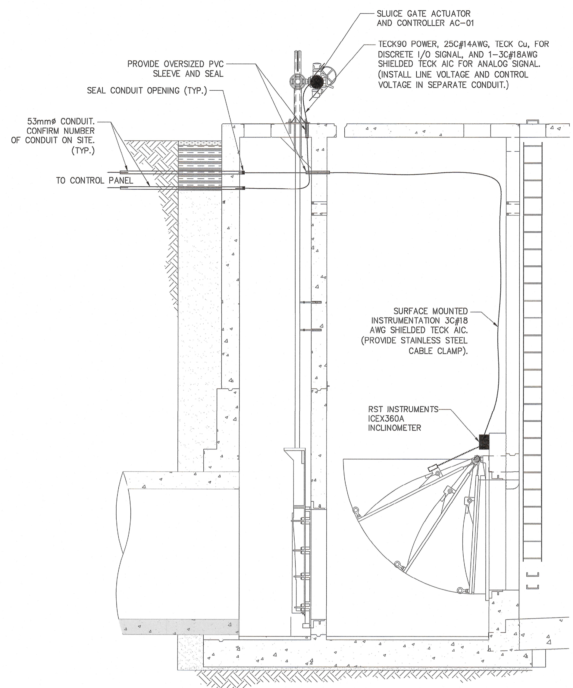
3 GATE CHAMBER SCALE: NTS
