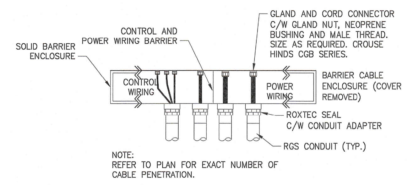
4 WIRING TO CONTROL PANEL (TYP.) SCALE: NTS
