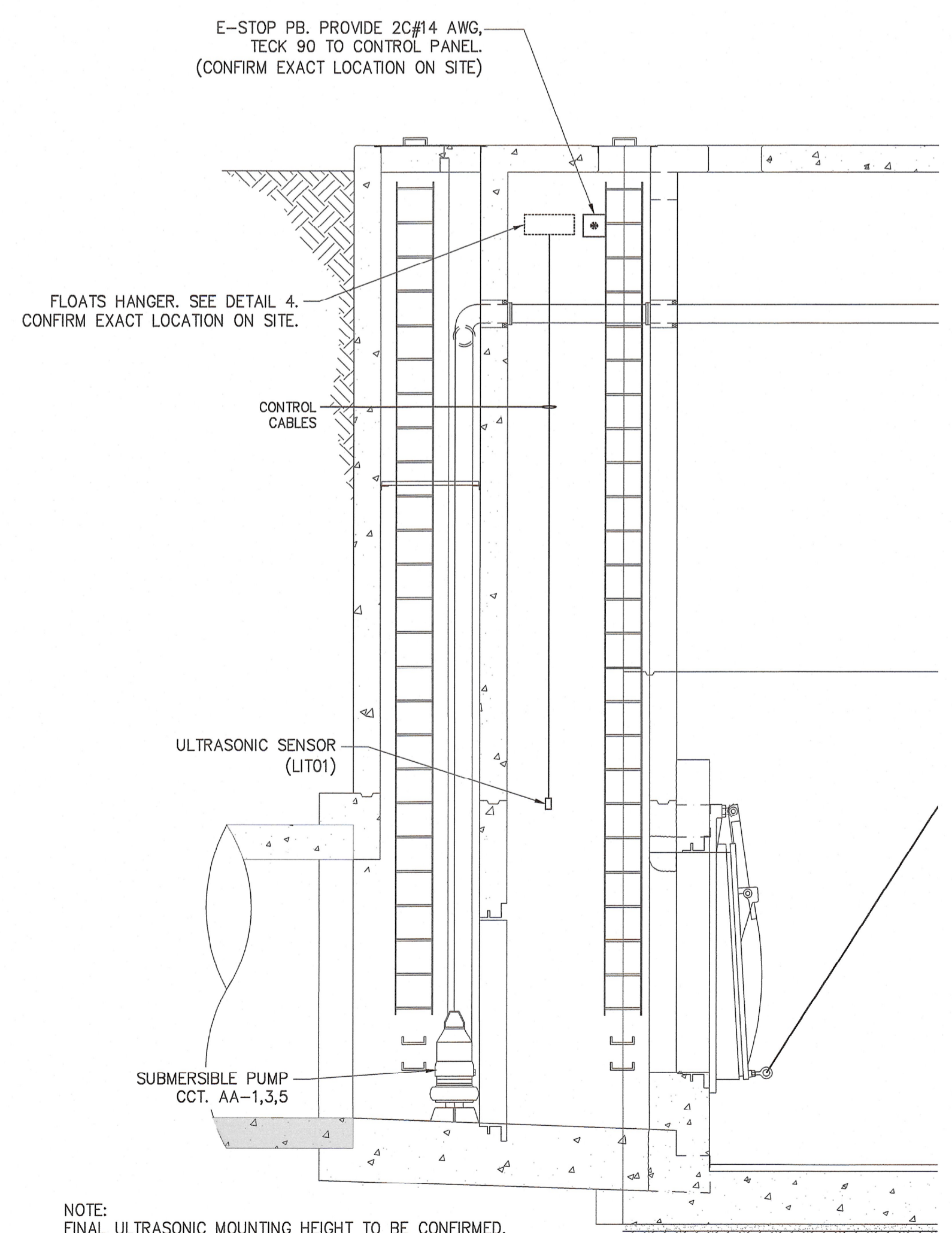
2 SUBMERSIBLE PUMP CHAMBER SCALE: NTS
