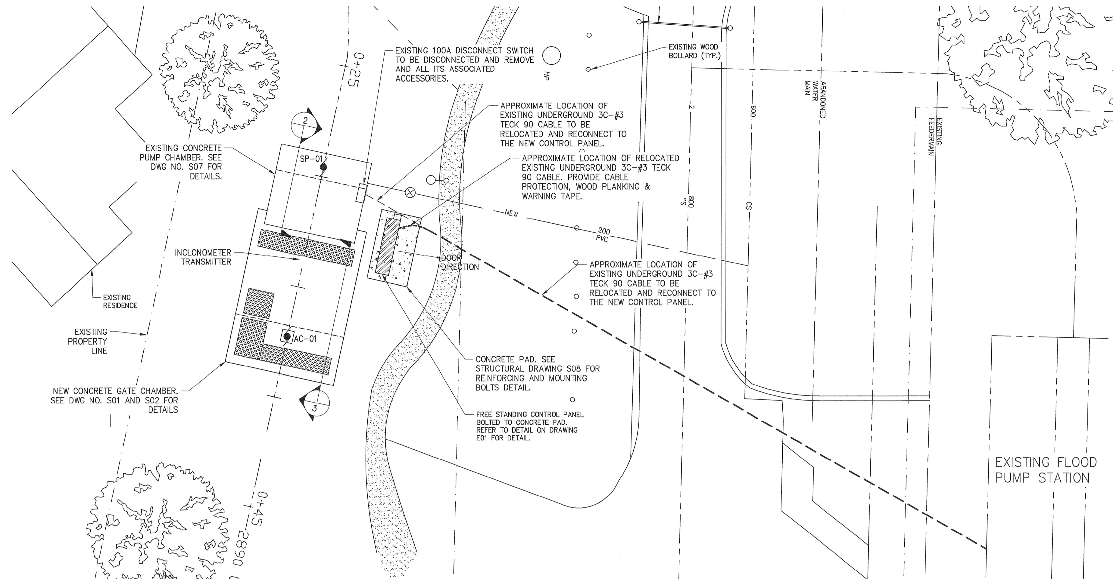
1 ELECTRICAL SITE PLAN SCALE: 1:100
