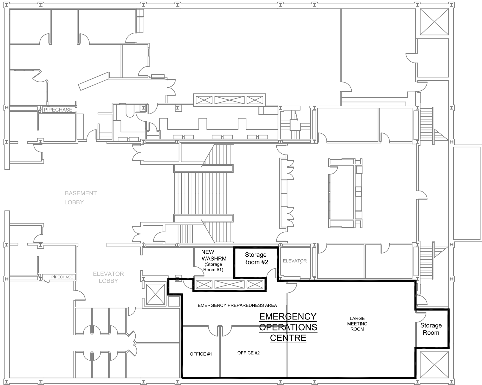
Council Building - Basement - EOC 510 Main Street (not to scale)
