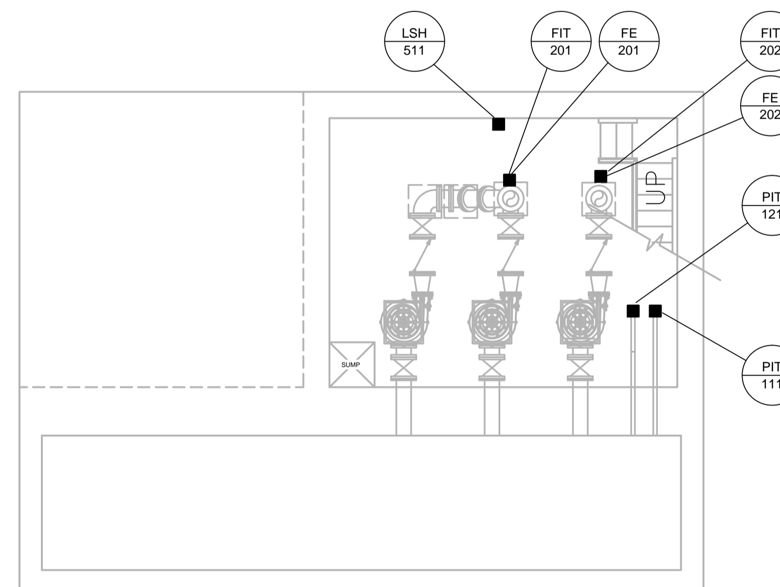
PUMP ROOM FLOOR PLAN 1:50
