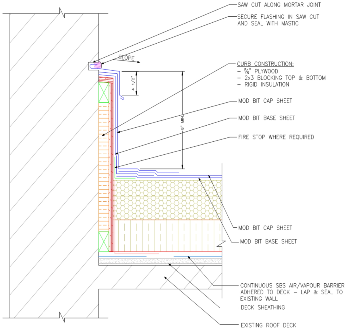
TYPICAL MASONRY DETAILS
