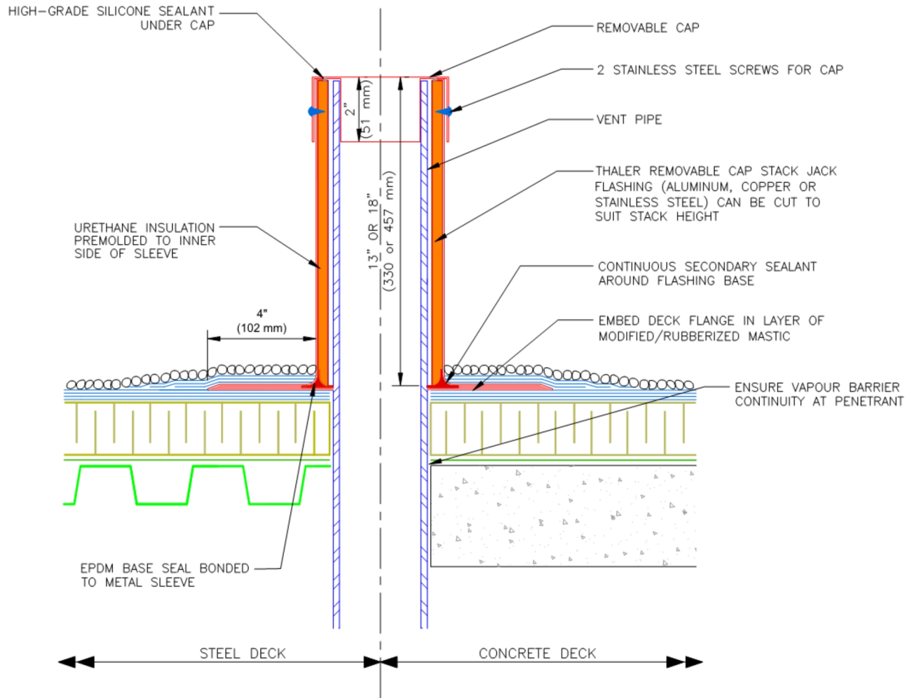
REMOVABLE CAP STACK JACK™ FLASHING (Insulated) PATENTED
