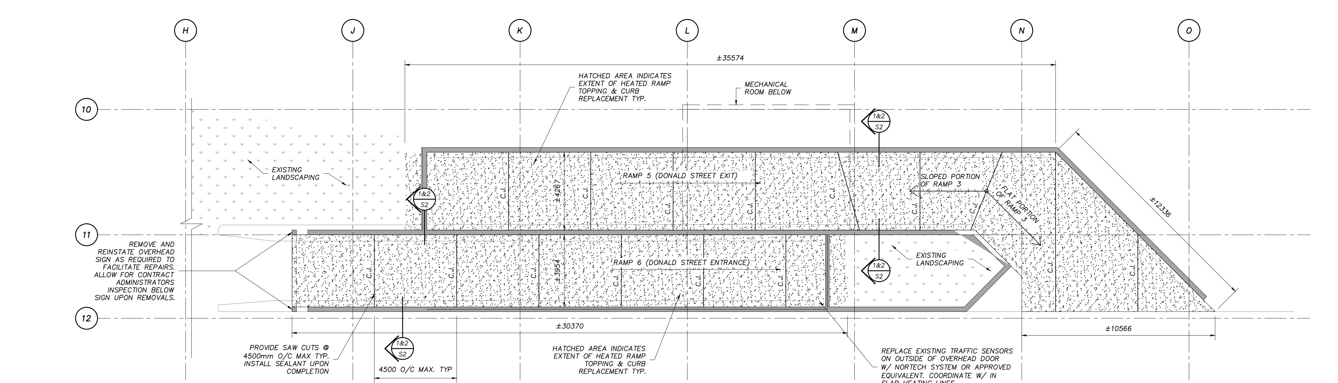
2 PARTIAL STREET LEVEL PLAN - DONALD STREET RAMPS SCALE: 1:125
