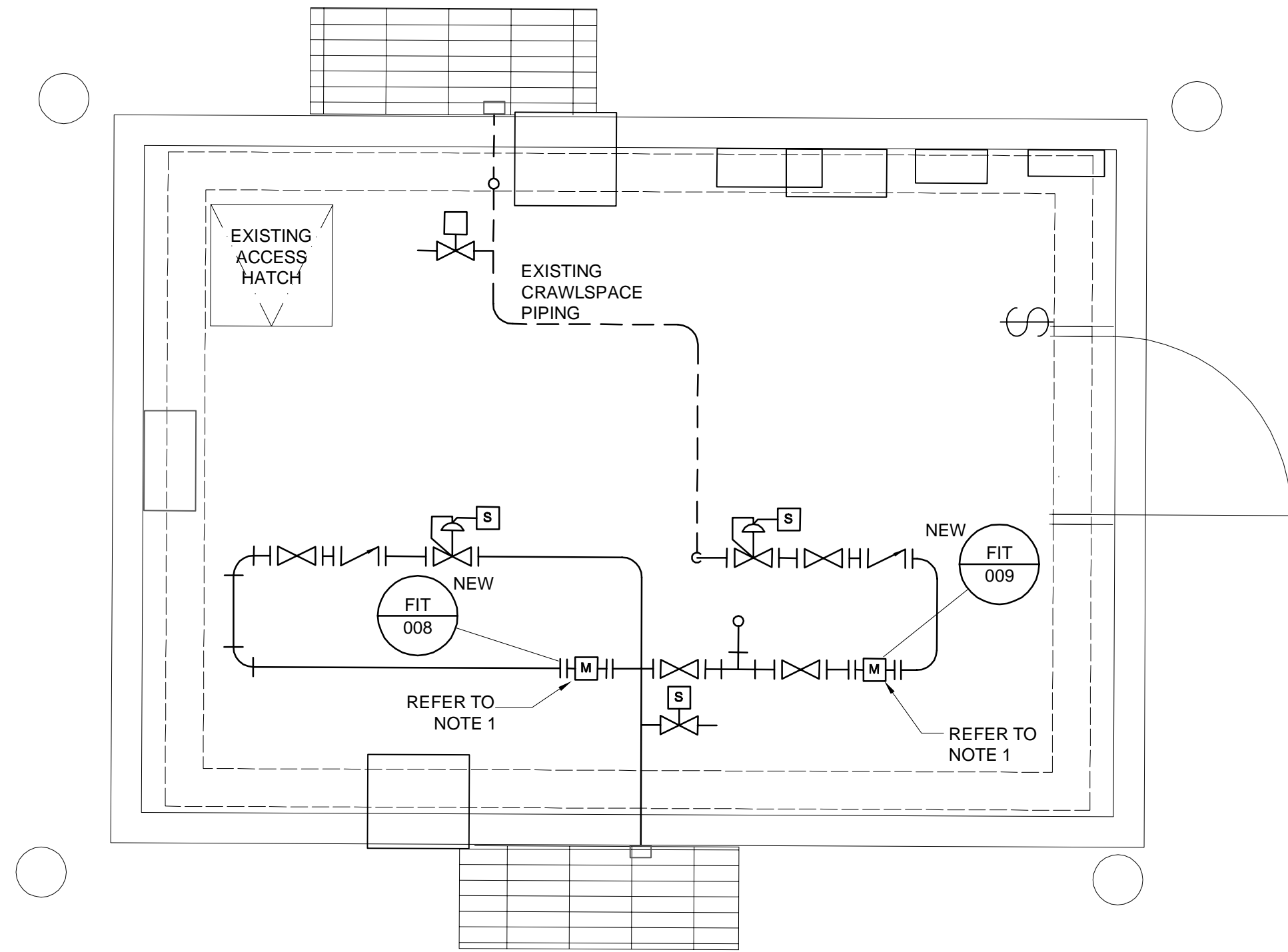
NEW BUILDING INSTRUMENTATION PLAN SCALE 1:25
