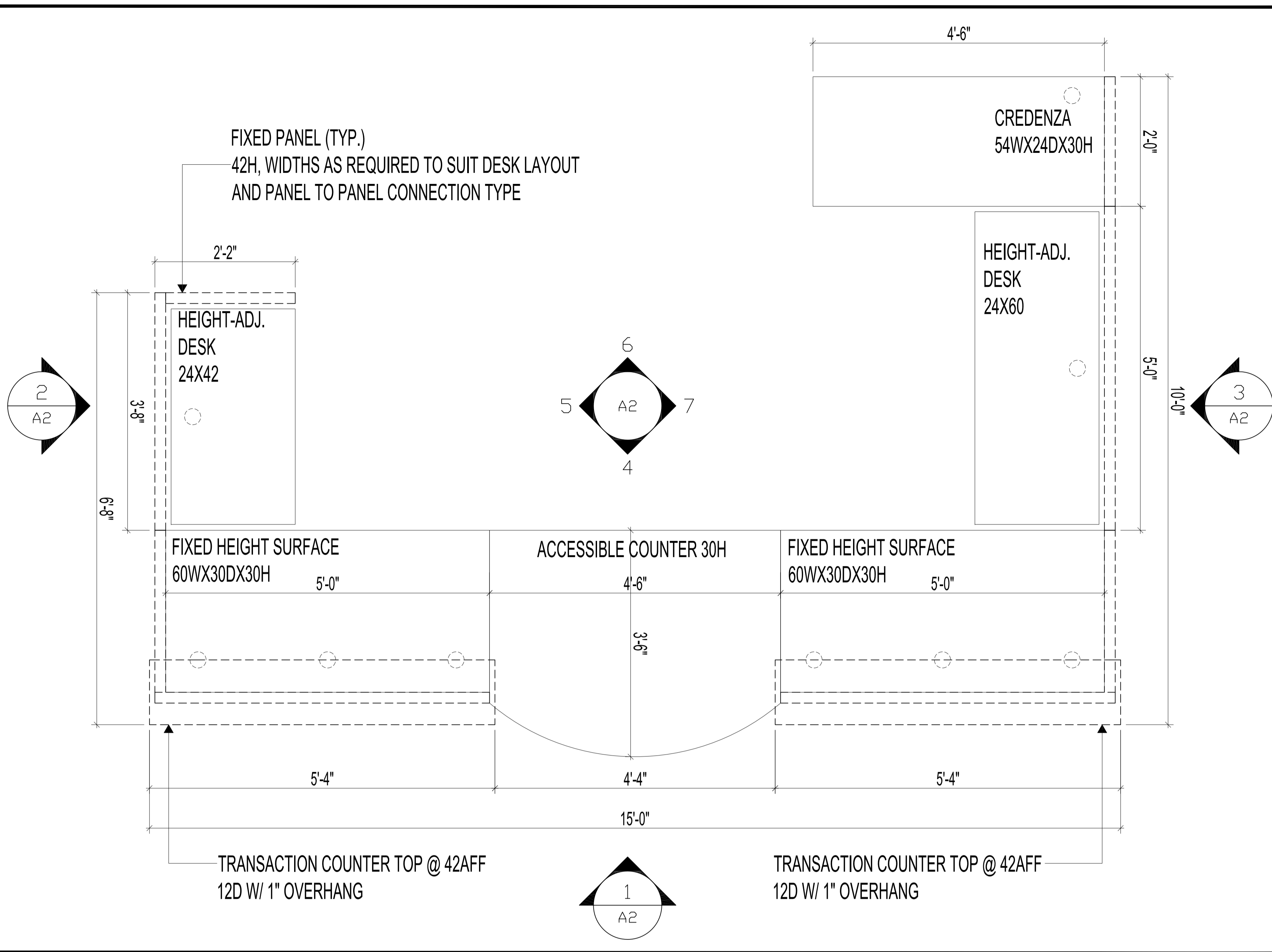
RECEPTION DESK PLAN SCALE: 1"=1'-0"
