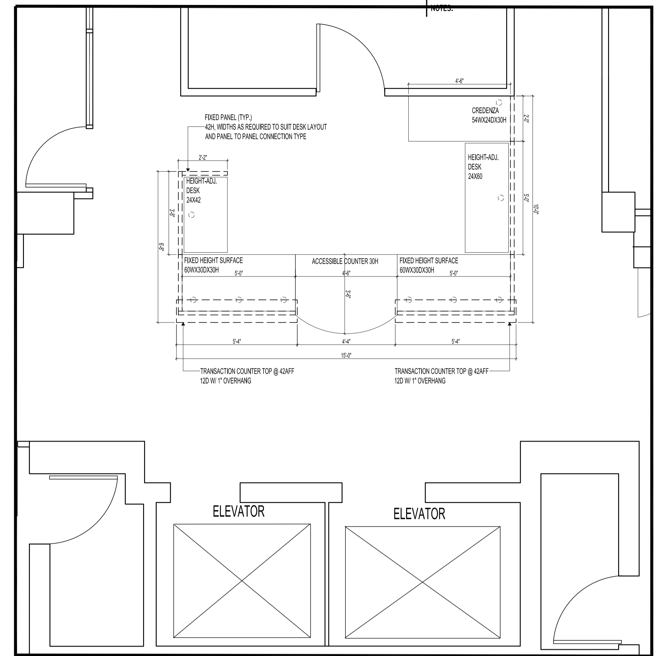
PARTIAL FOURTH FLOOR PLAN SCALE: 3/8"=1'-0"
