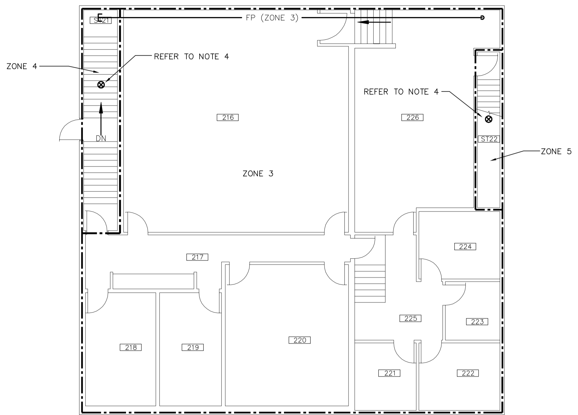
2 FIRE ALARM PLAN SECOND FLOOR TRAINING CENTRE 1 : 100
