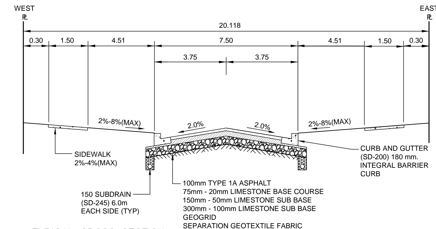
TYPICAL CROSS SECTION N.T.S.
