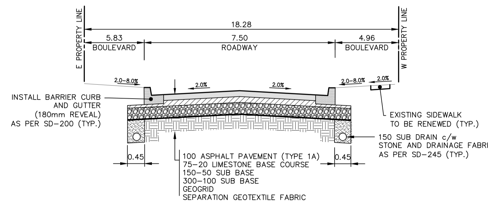
TYPICAL CROSS-SECTION
