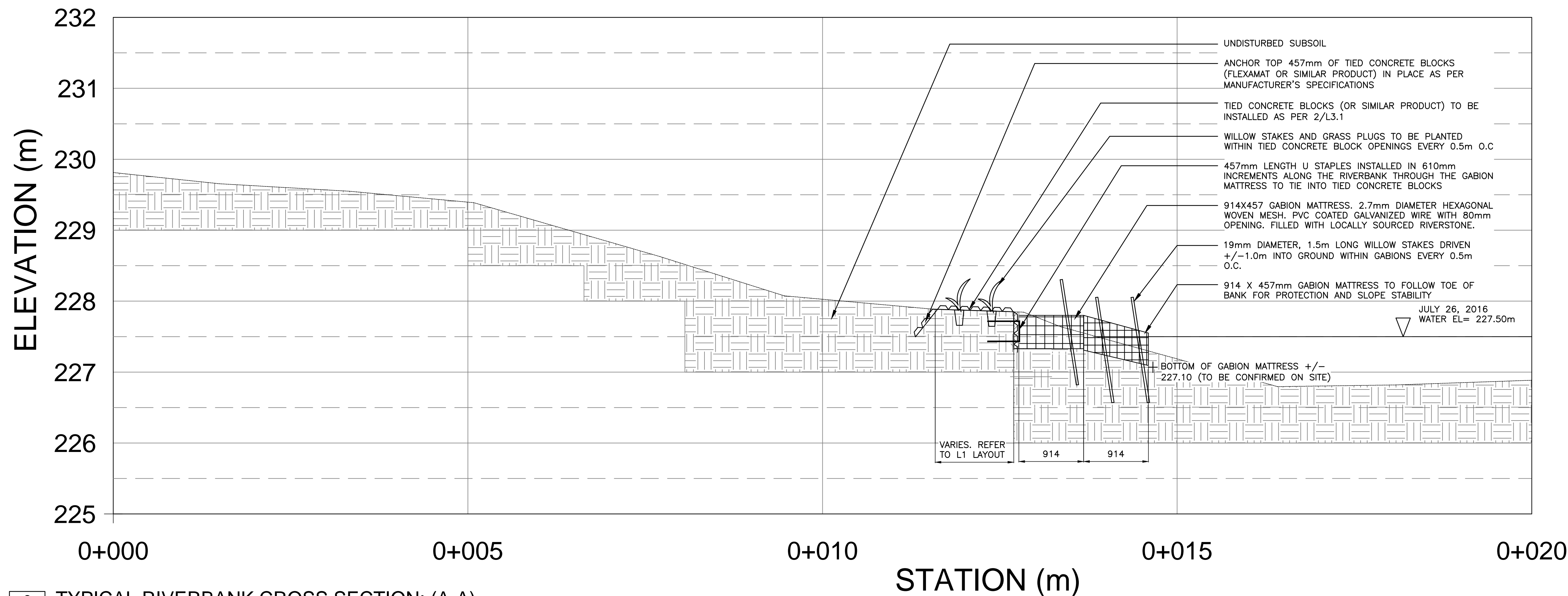
6 TYPICAL RIVERBANK CROSS SECTION: (A-A) L3.2
