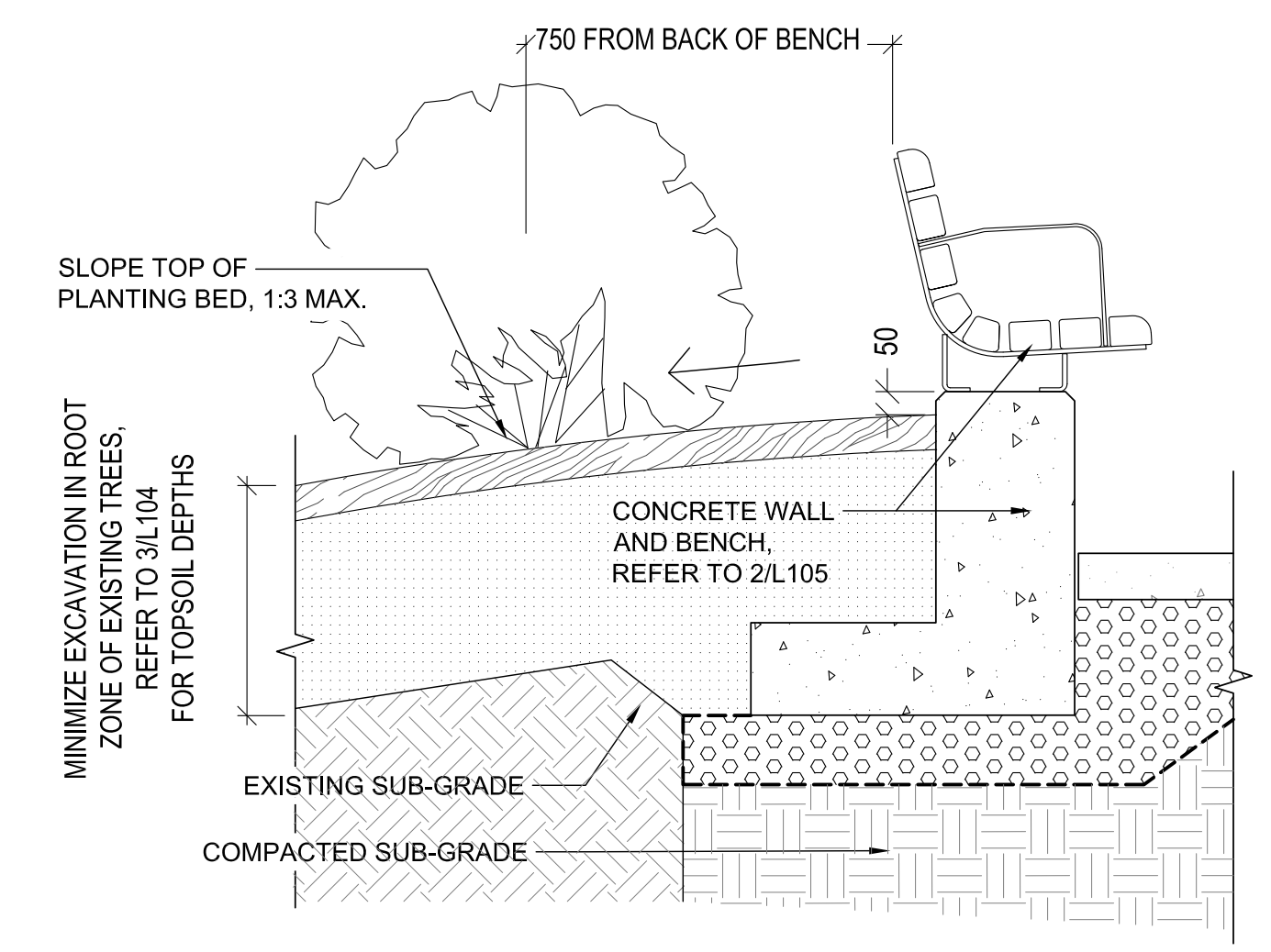
2 SLOPED PLANTING BED SCALE - 1 : 15 AT 24"x36"
