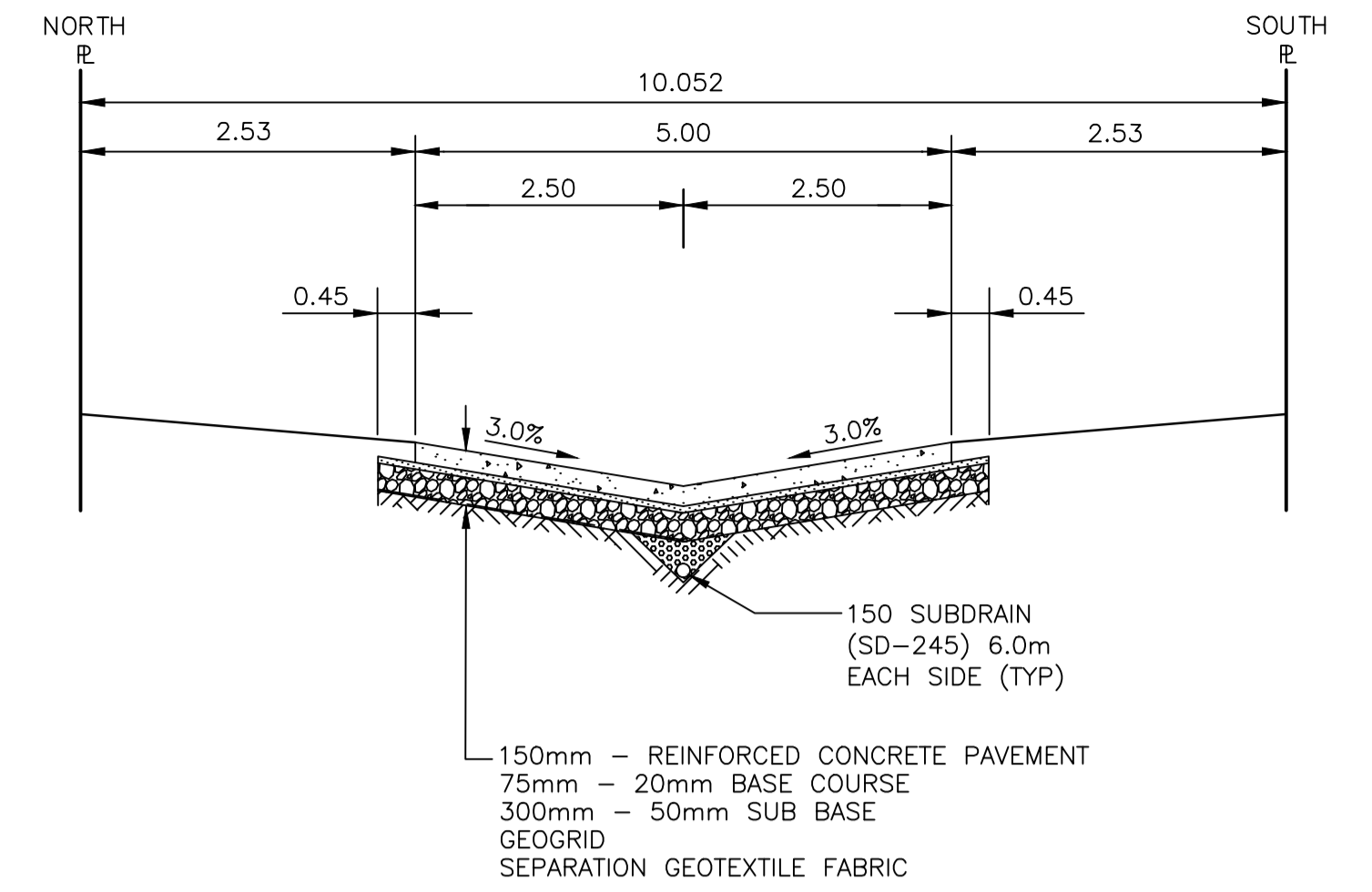
TYPICAL CROSS SECTION N.T.S.
