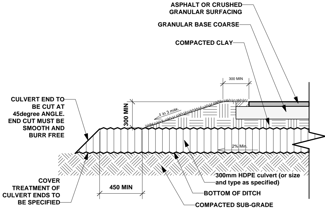
SECTION THROUGH PATH AND CULVERT
