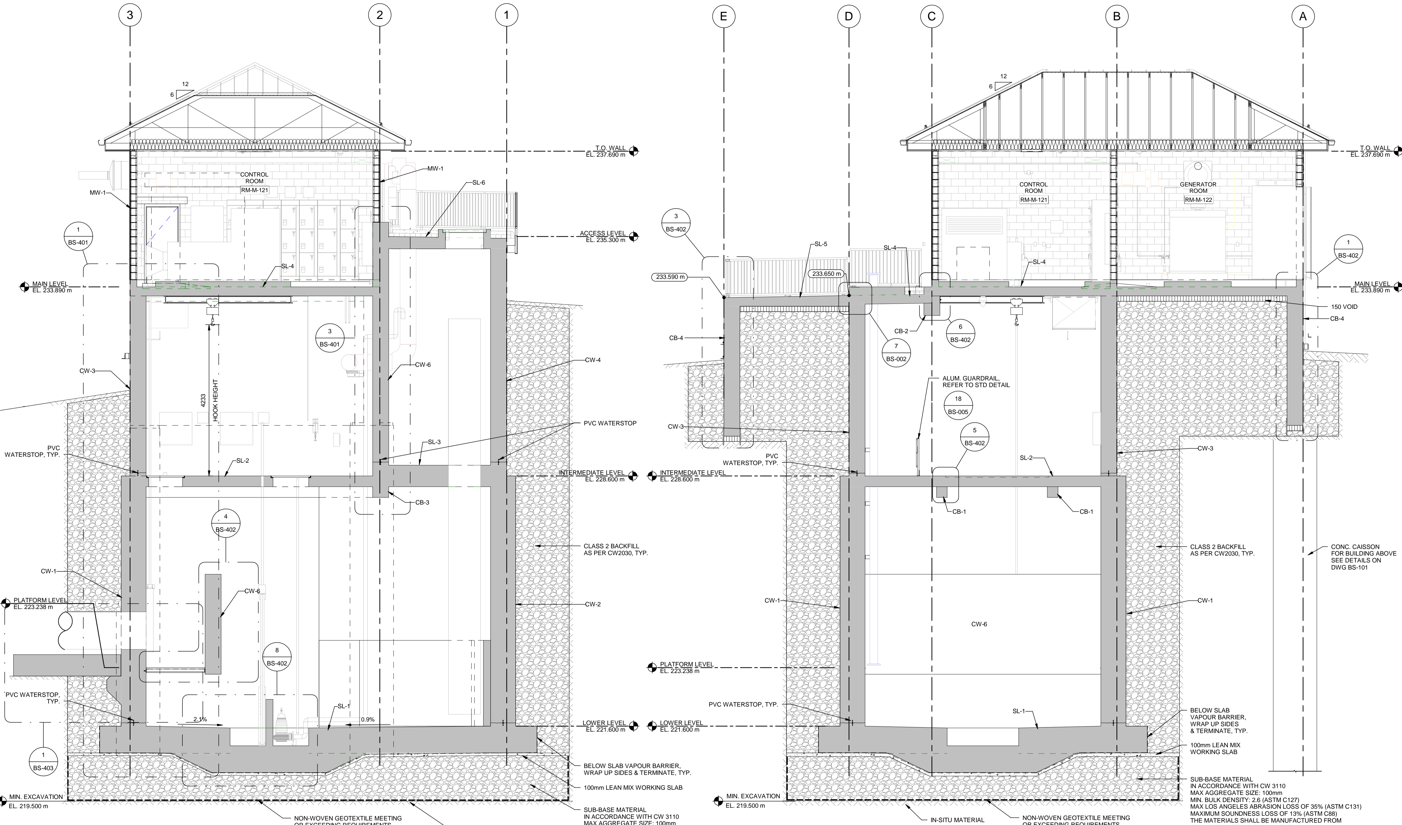
A SECTION BS-301 REF: BS-101 SCALE: 1:50
