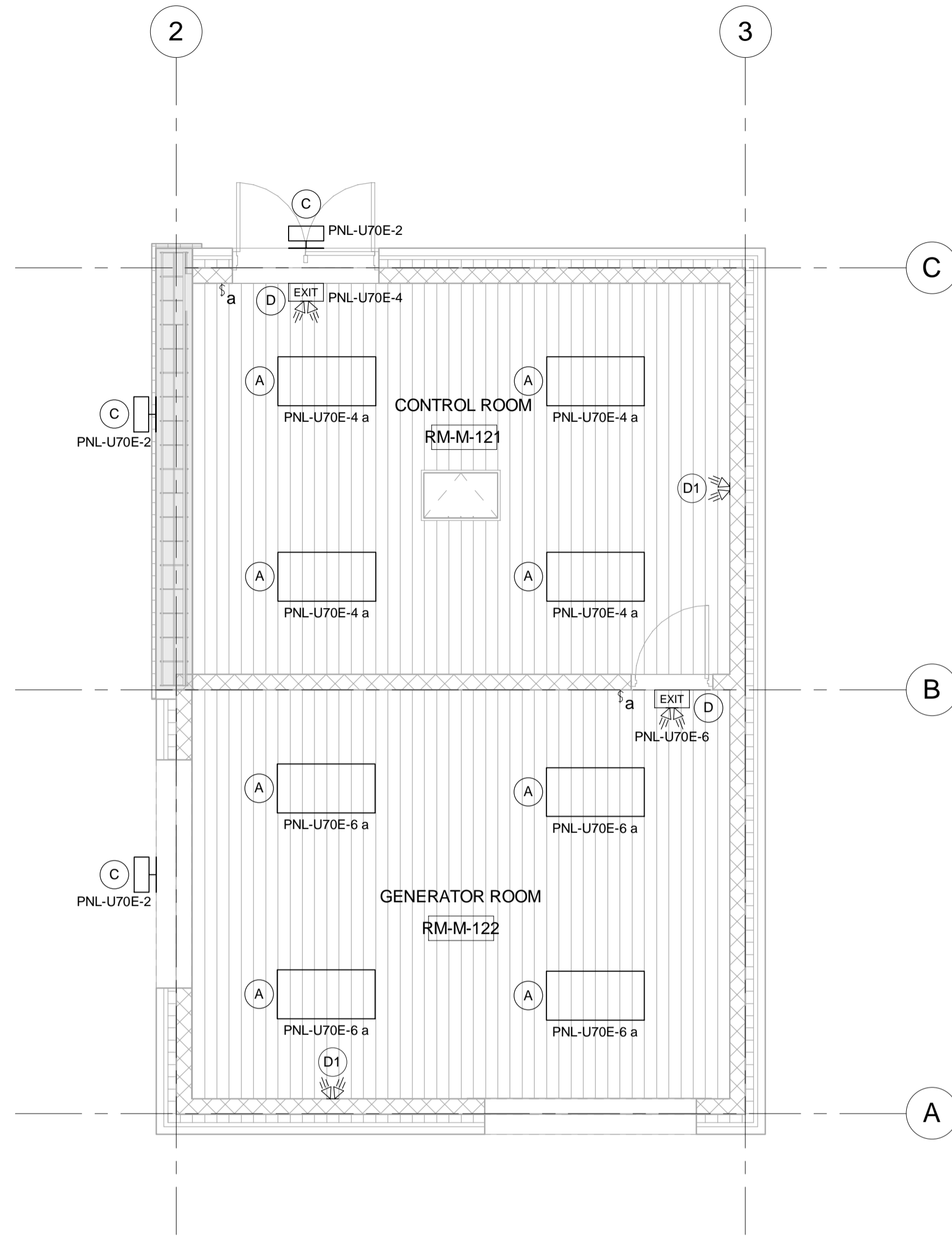
1 MAIN LEVEL - LIGHTING PLAN
