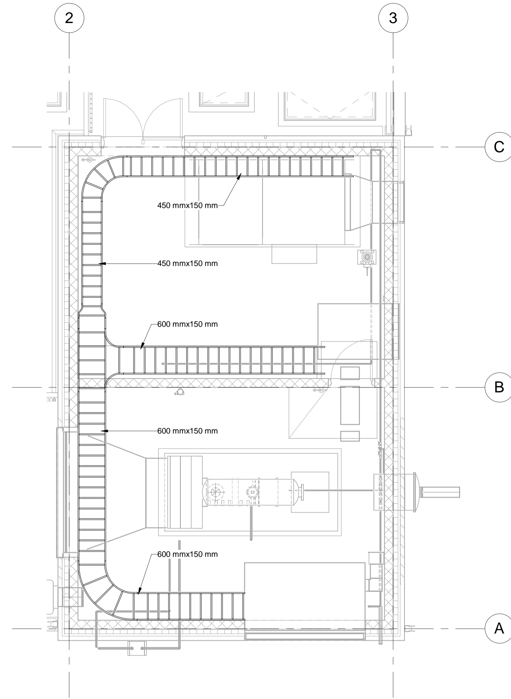
2 MAIN LEVEL - CABLE TRAY
