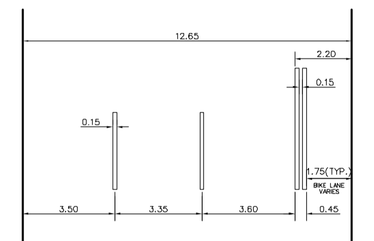
TYPICAL LANE LINE MARKING SECTION NTS
