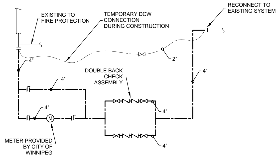
1 DETAILS - NEW INCOMING WATER SERVICE DETAIL M1.4 SCALE: 1 : 1
