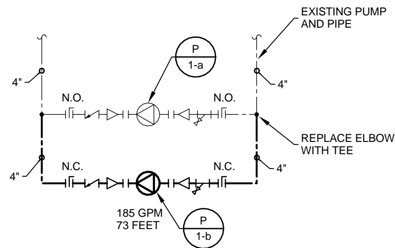
2 DETAILS - ADDITIONAL PUMP M1.4 SCALE: 1 : 1
