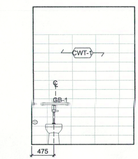
12 FEMALE W/C 117 A-402 1:50
