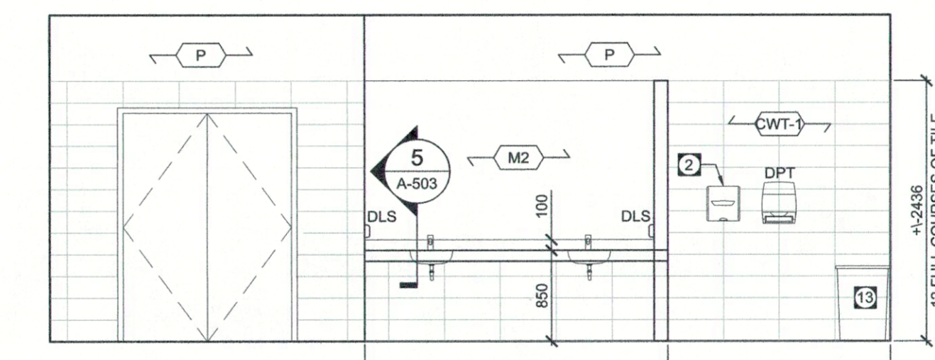
10 FEMALE W/C 117 A-402 1:50
