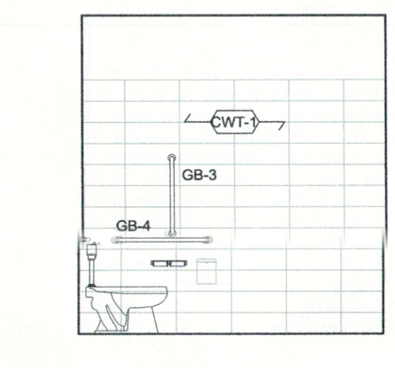
13 FEMALE W/C 117 A-402 1:50
