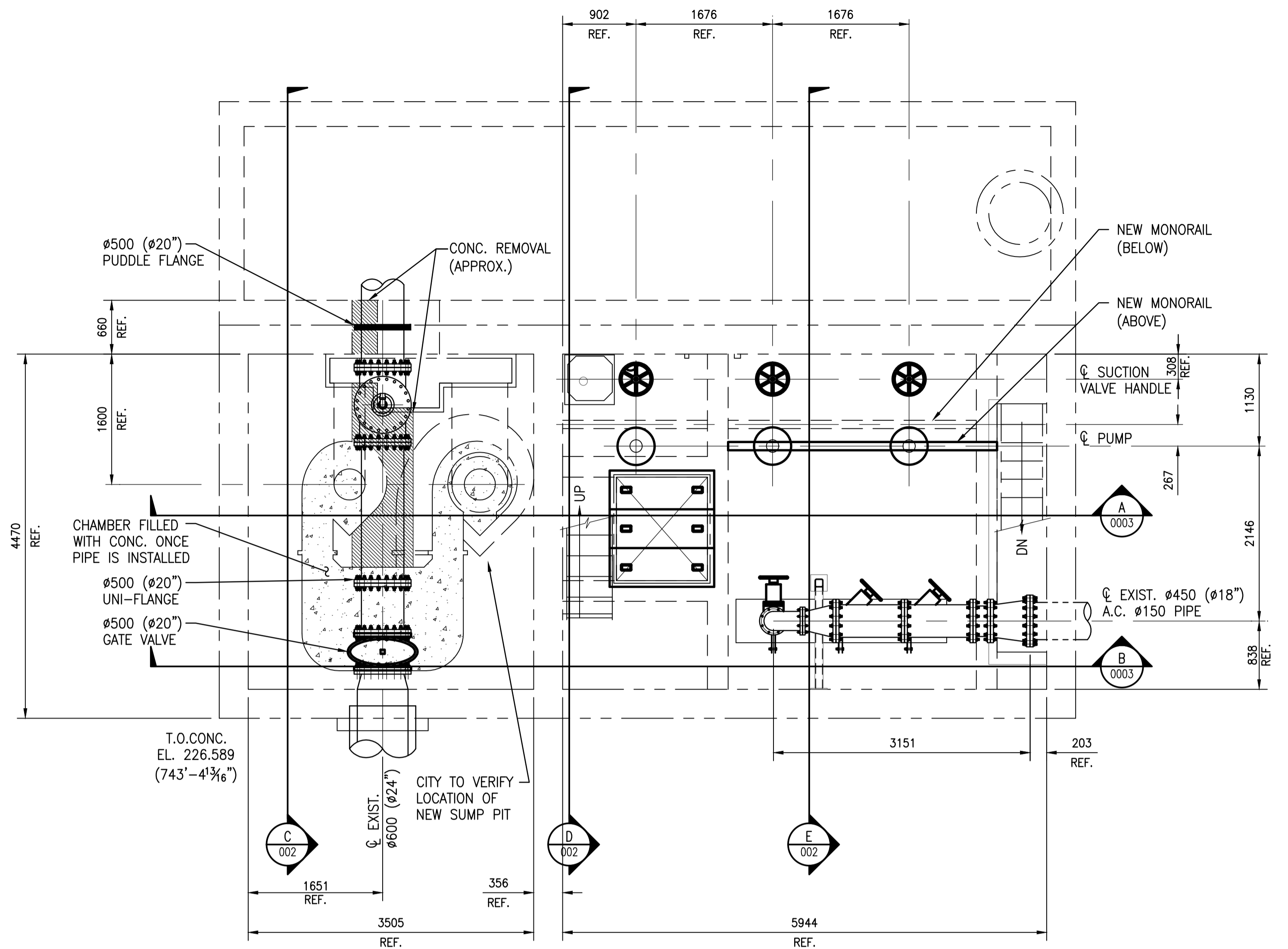
PLAN ABOVE EL. 227.635 (746'-10") SCALE: 1 : 40
