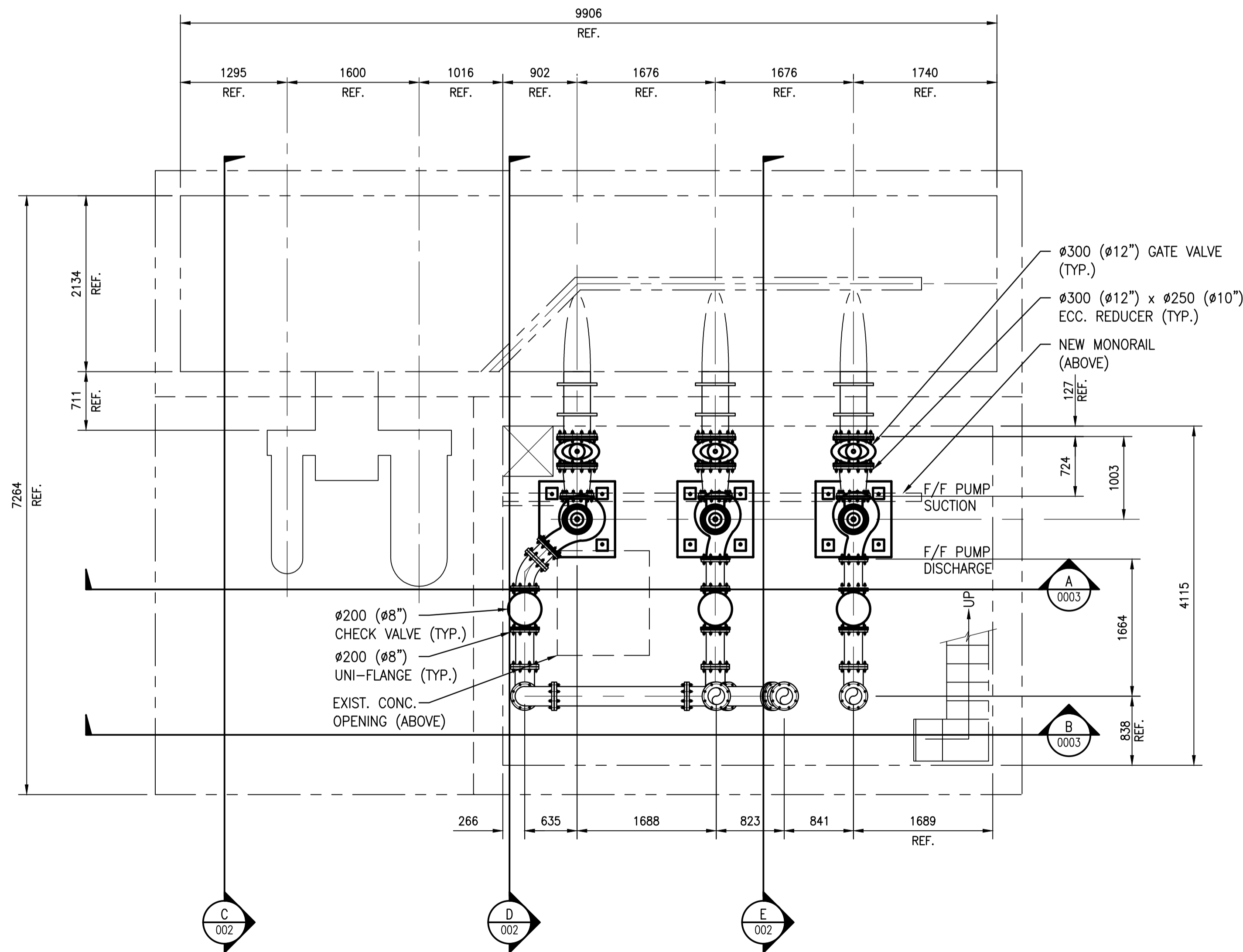
PLAN ABOVE EL. 224.269 (735'-9 1/2") SCALE: 1 : 40
