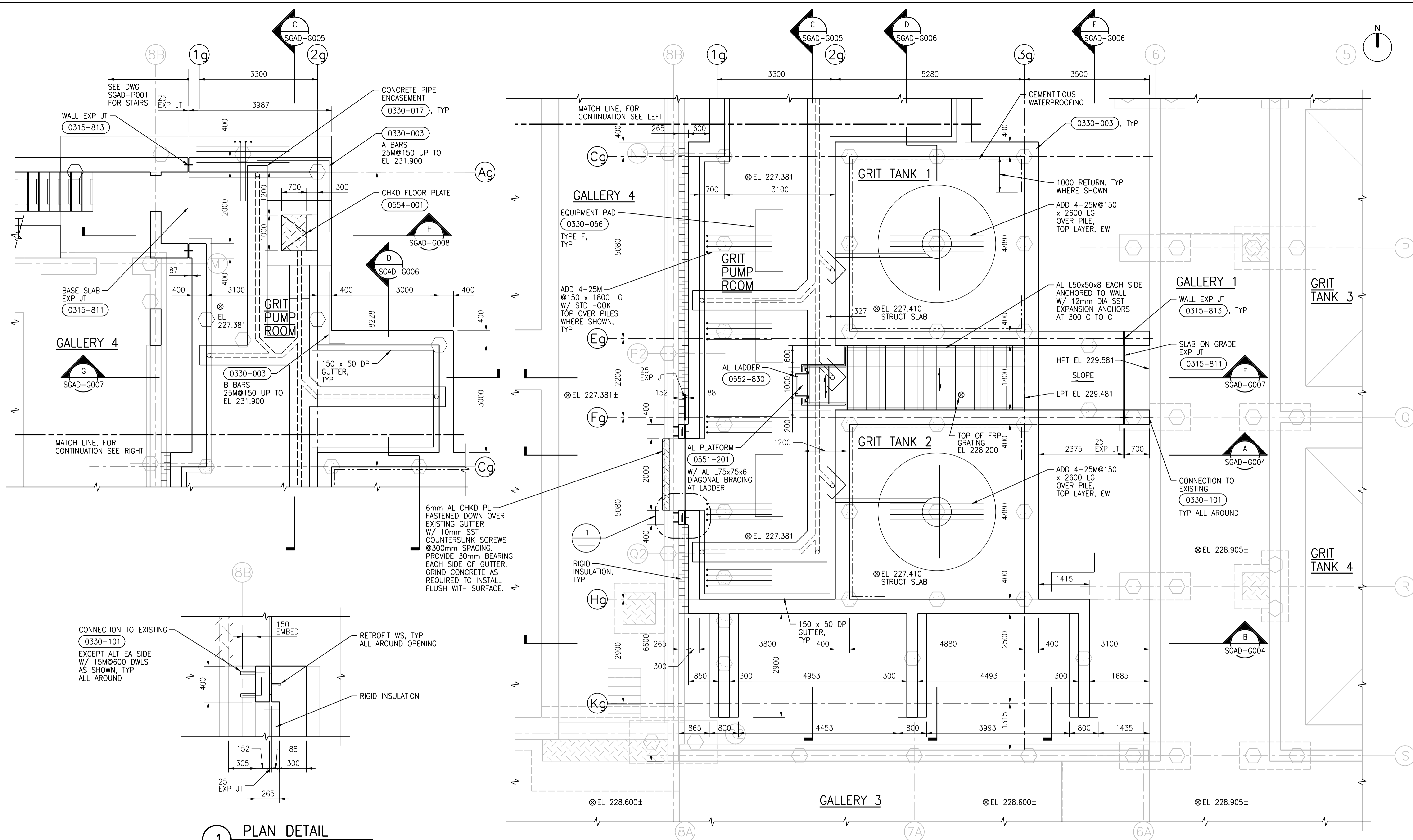
BASEMENT PLAN 1:50
