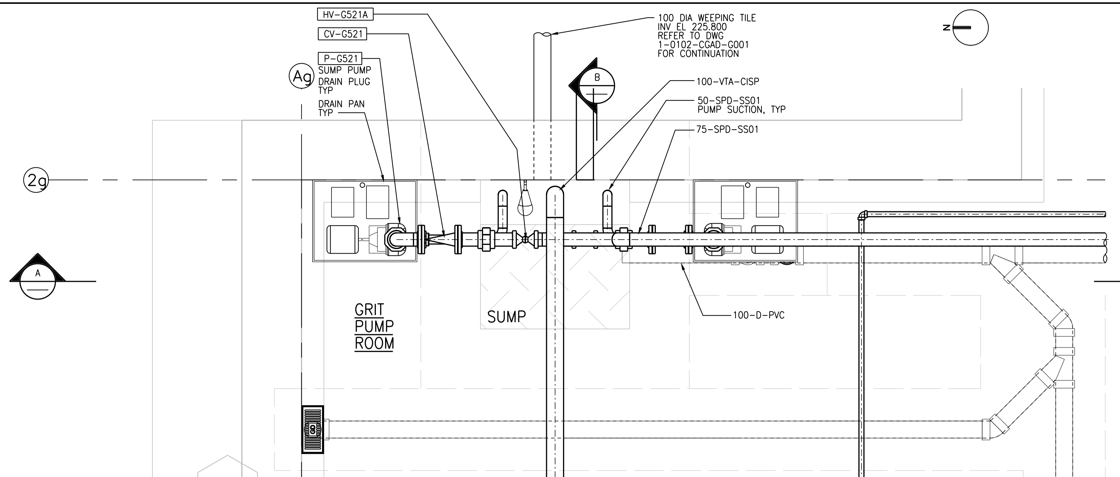
1 DETAIL 1:15 1-0102-MGAD-G501
