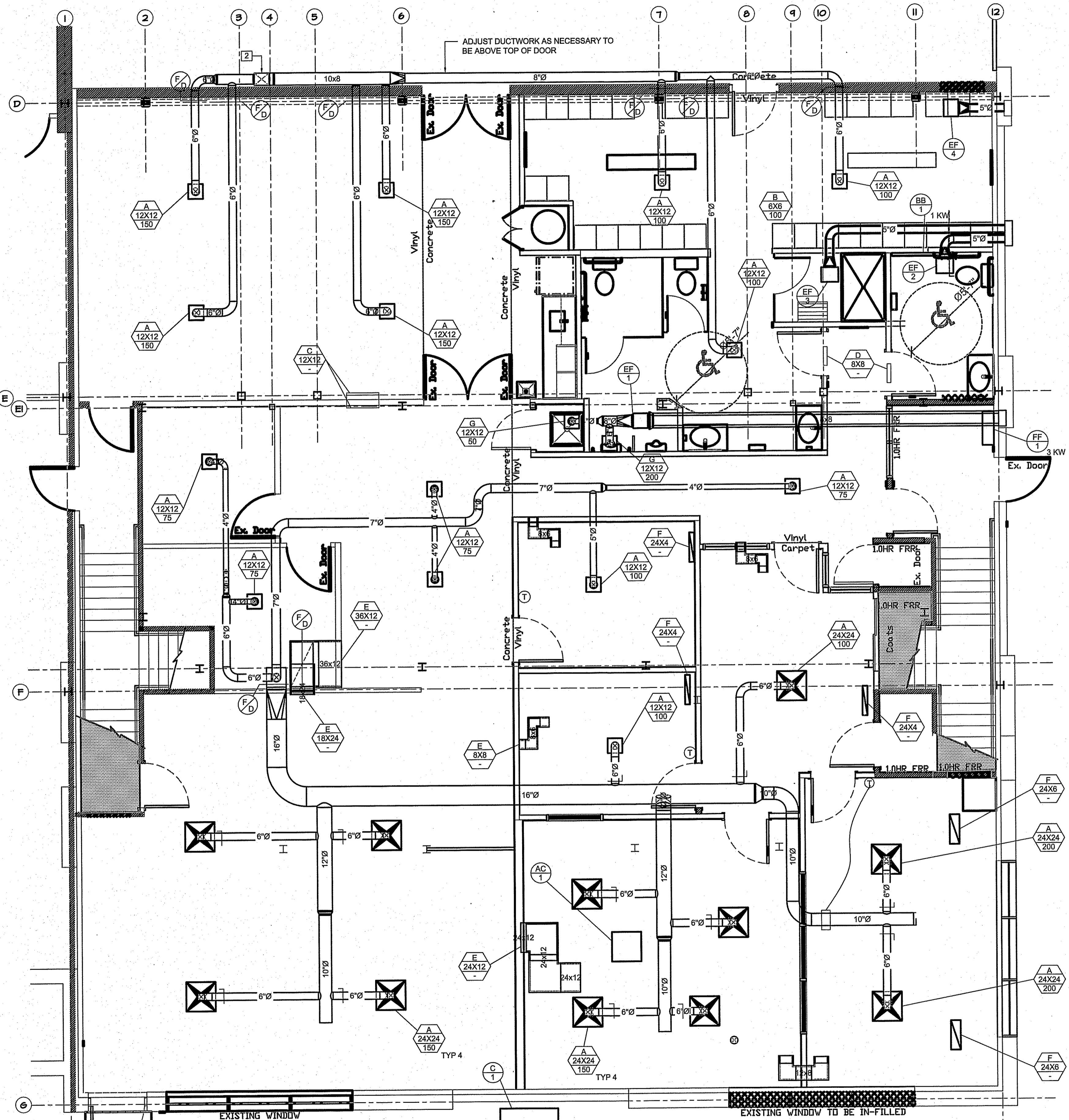
1 MAIN FLOOR PLAN - HVAC M2.0 SCALE: 1/4"=1'-0"
