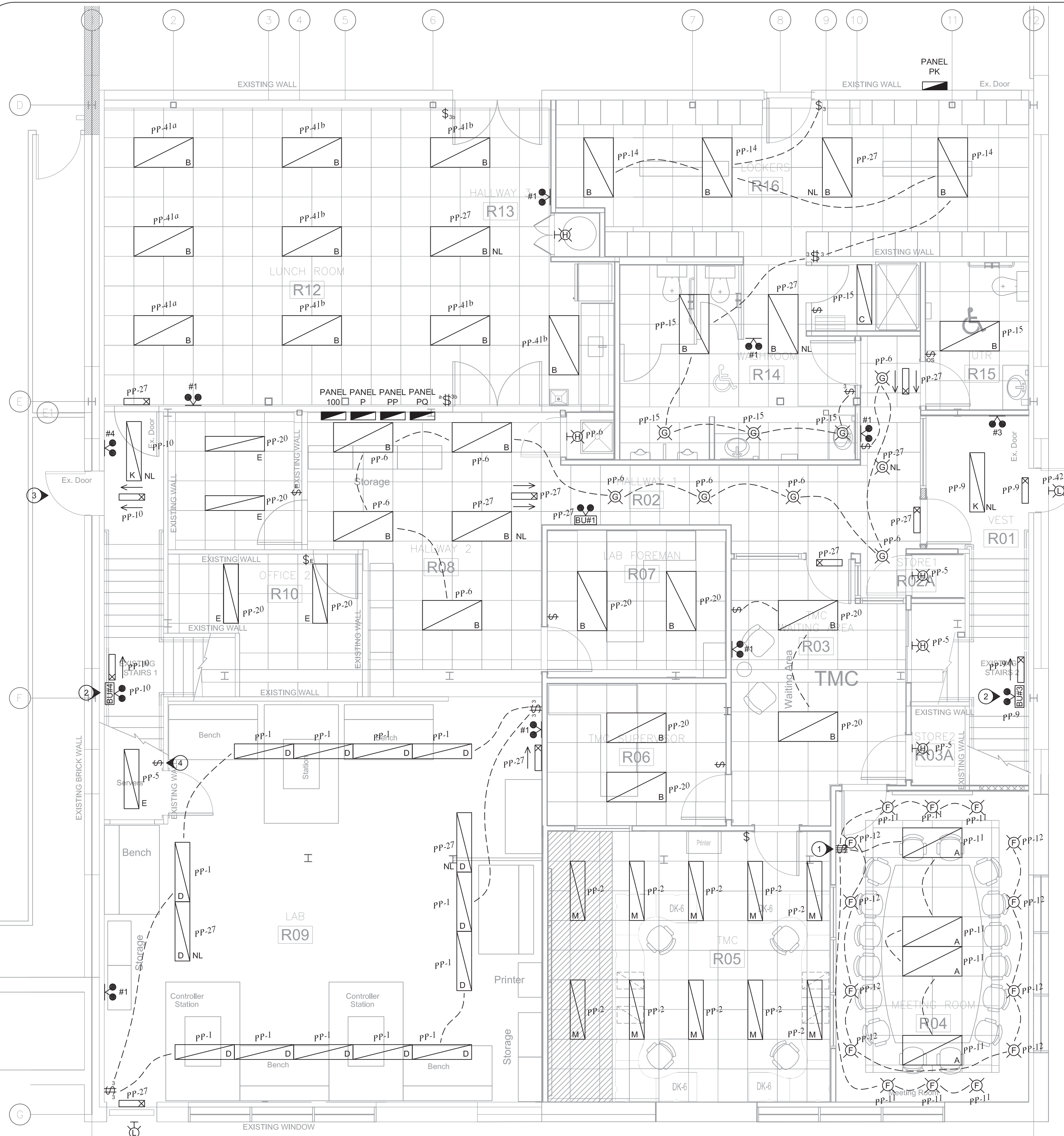
1 MAIN FLOOR LIGHTING PLAN SCALE: 1/4" = 1' - 0"
