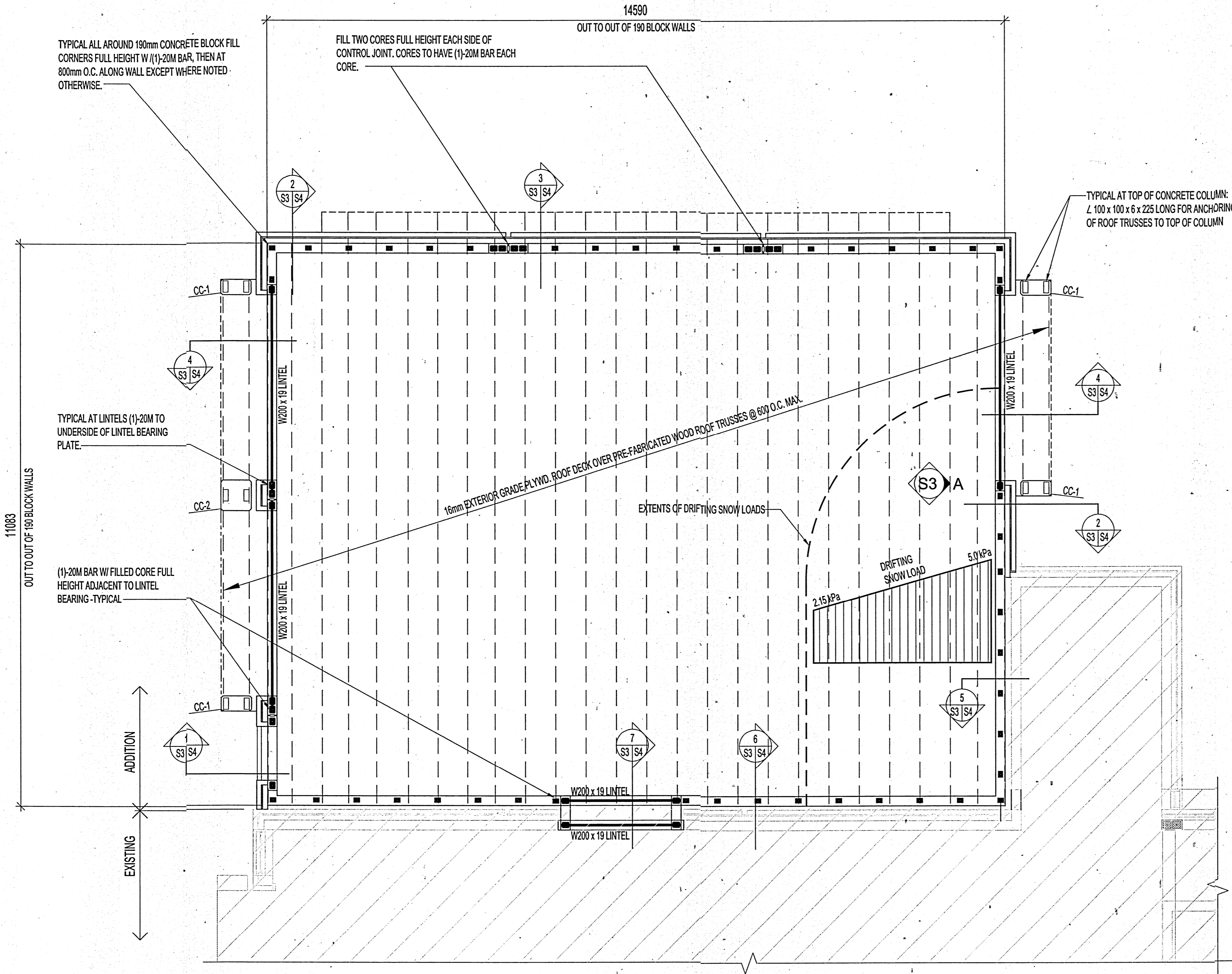
1 S3 ROOF FRAMING PLAN SCALE 1:50
