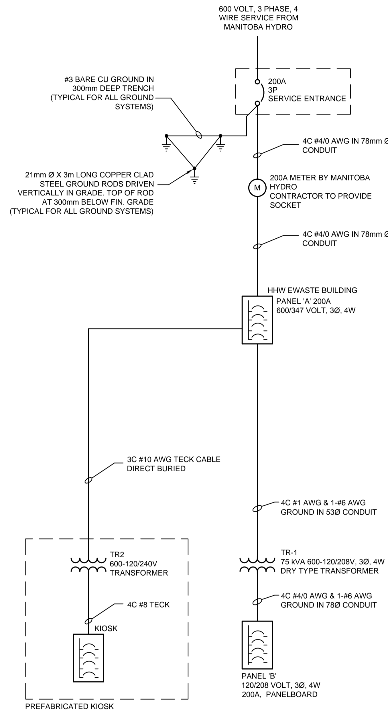
SINGLE LINE DIAGRAM
