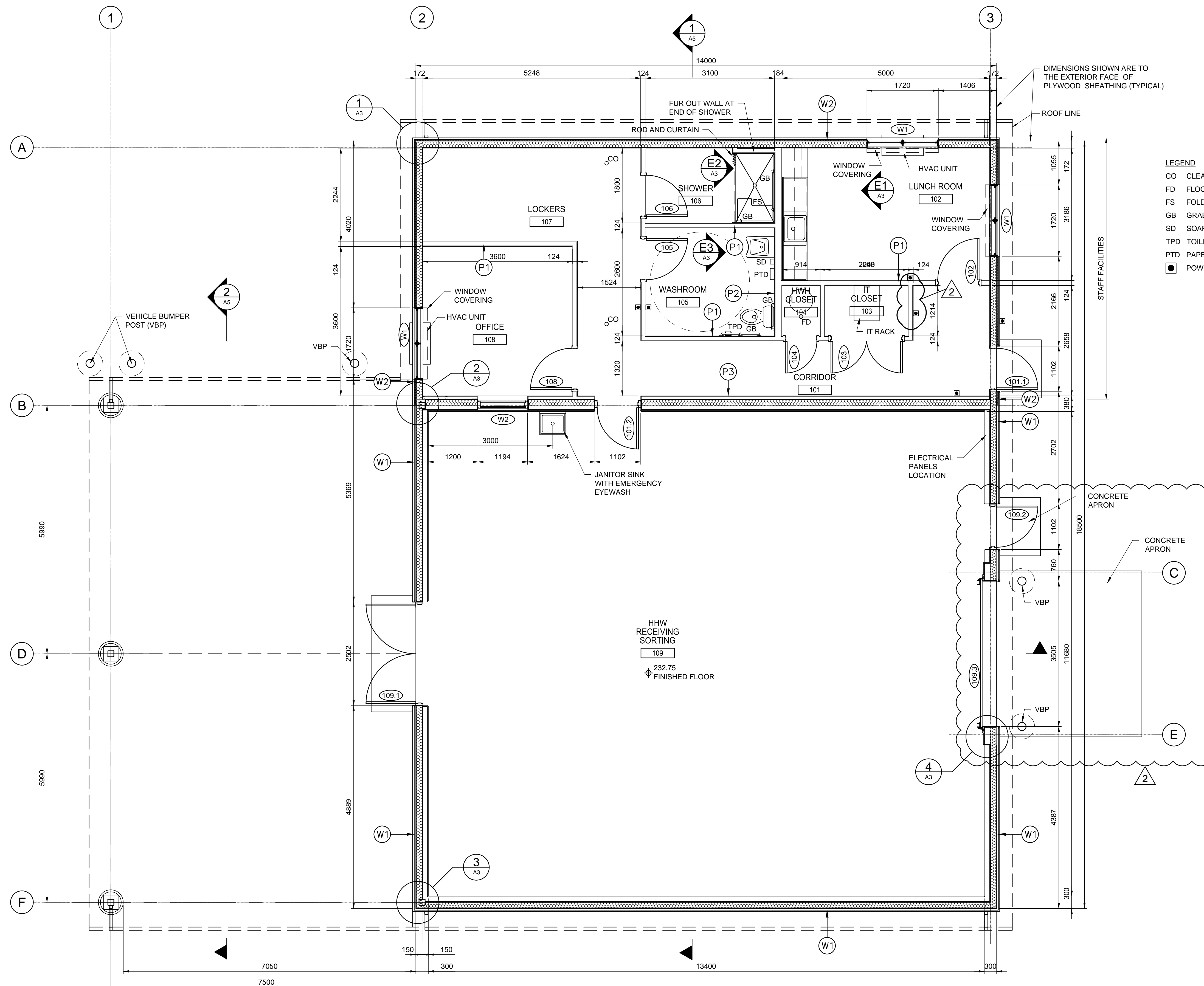
FLOOR PLAN 1:50
