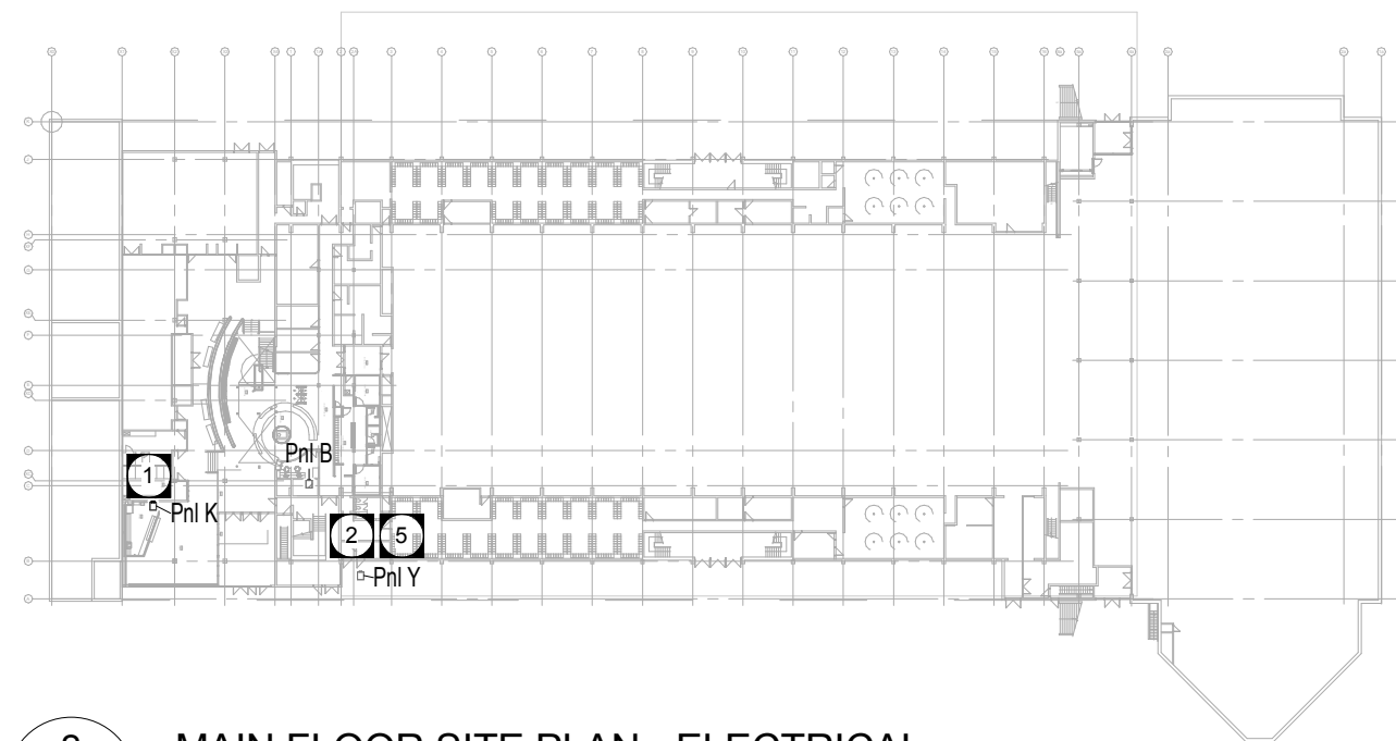
2 MAIN FLOOR SITE PLAN - ELECTRICAL DE-01 SCALE: 1 : 1000
