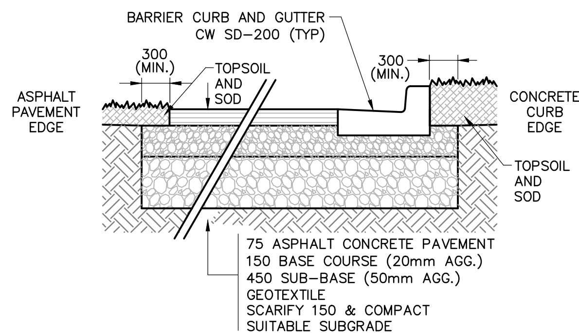
MEDIUM DUTY ASPHALT PAVEMENT STRUCTURE N.T.S.
