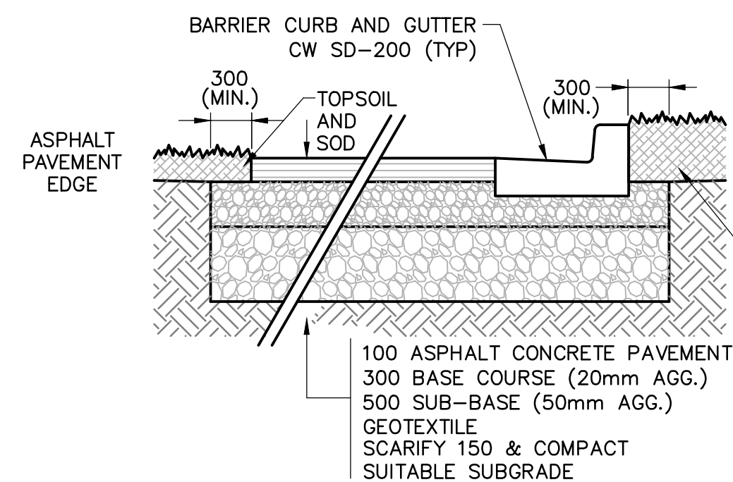
HEAVY DUTY ASPHALT PAVEMENT STRUCTURE N.T.S.
