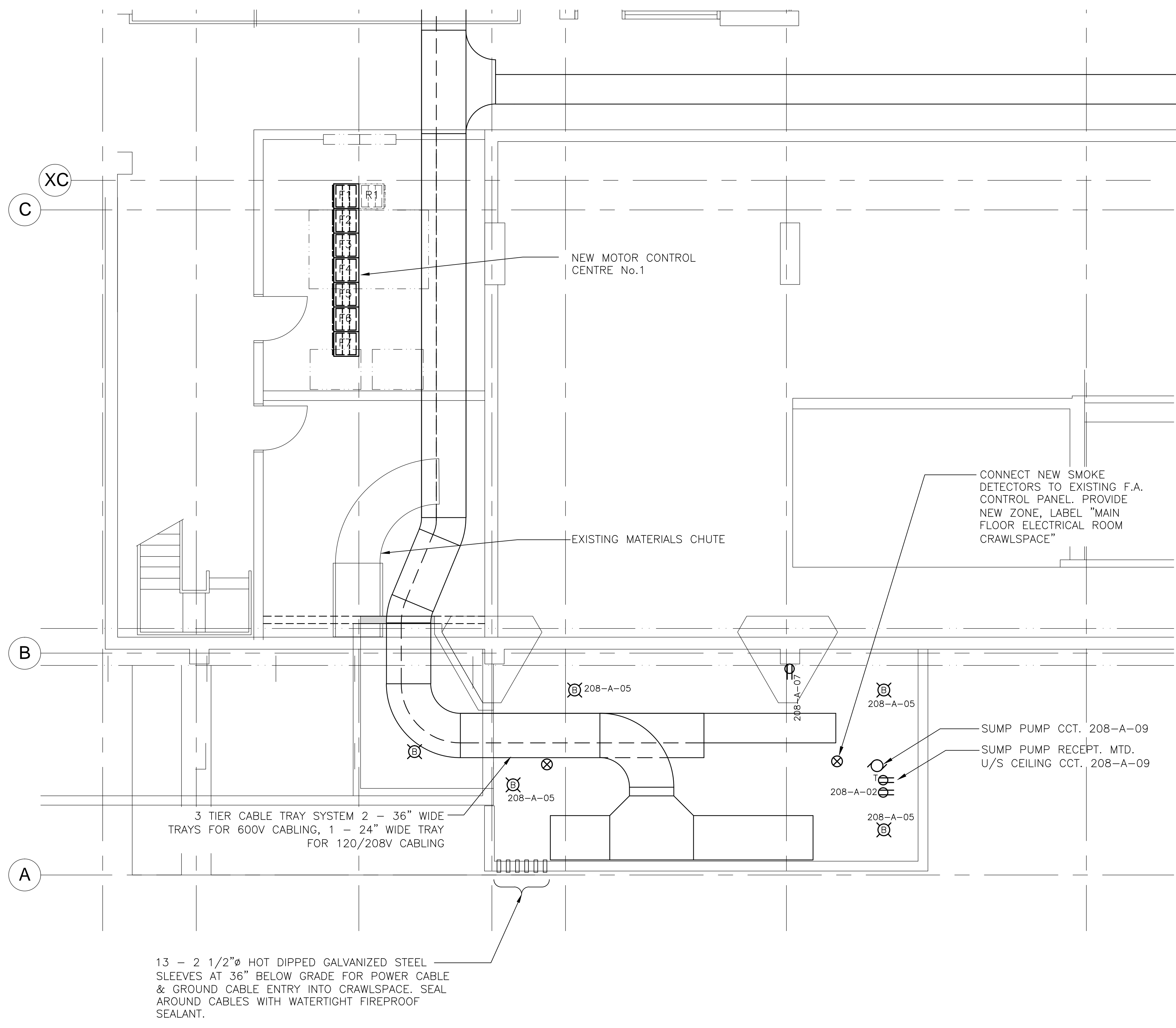
CRAWLSPACE LEVEL - ELECTRICAL ROOM 1/4" = 1'-0"
