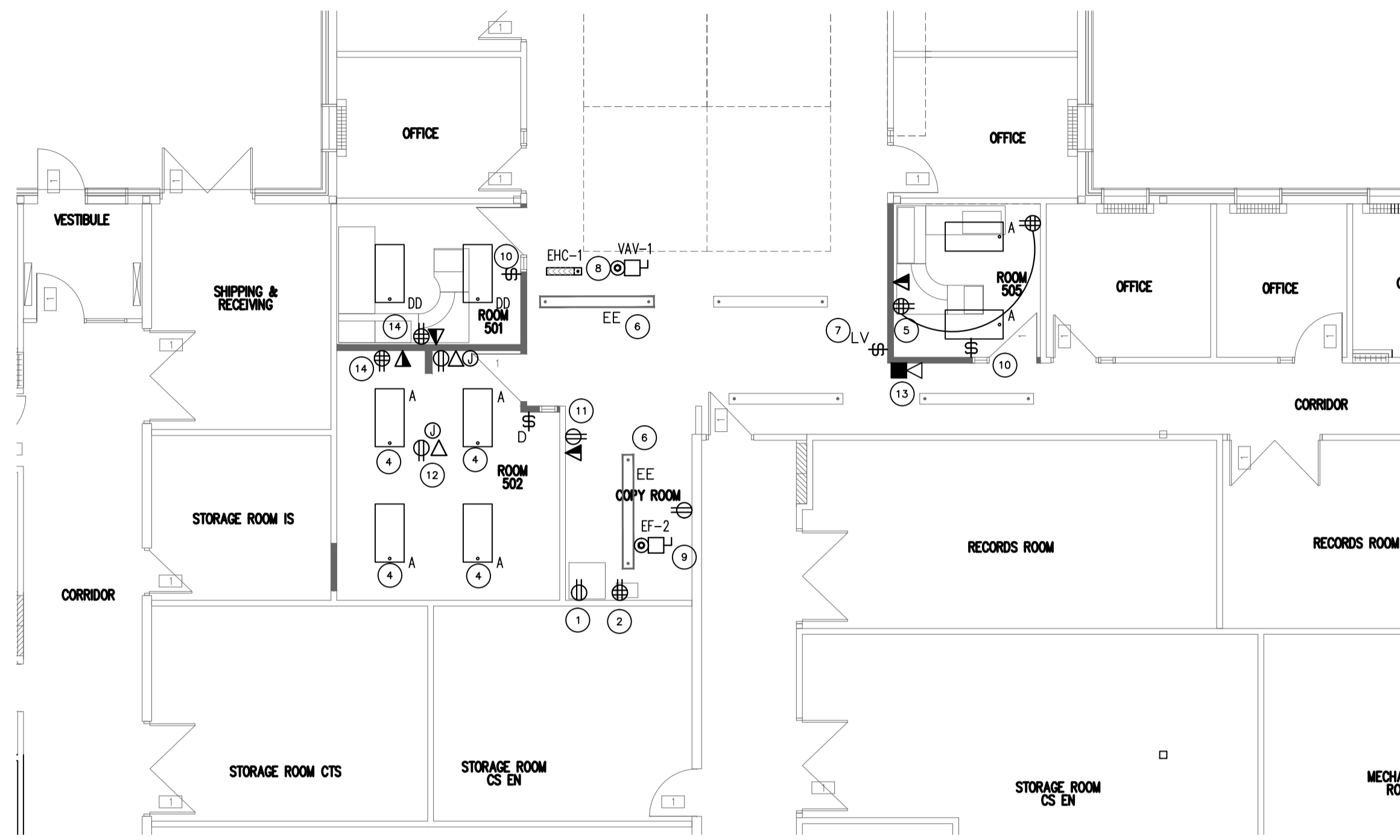
PARTIAL MAIN FLOOR PLAN-LIGHTING AND POWER-RENO SCALE: 1/8"=1'-0"
