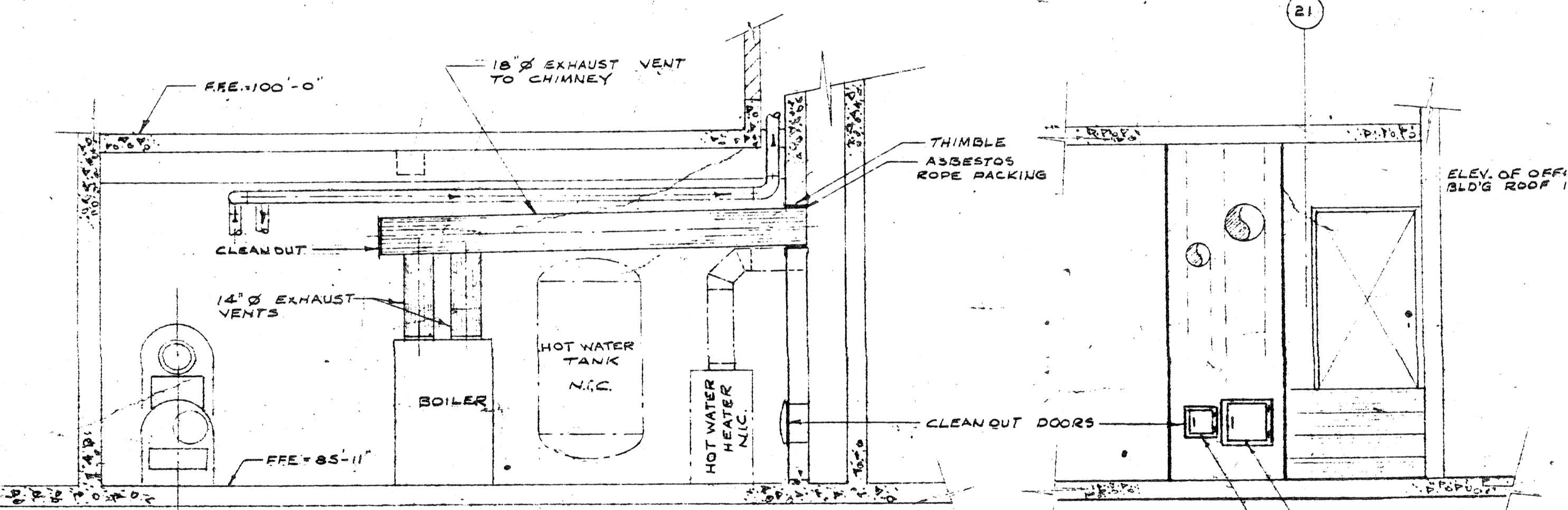
SECTION SHOWING CLEANOUT DOORS FOR EXHAUST CHIMNEY SCALE 1/4\"/>
