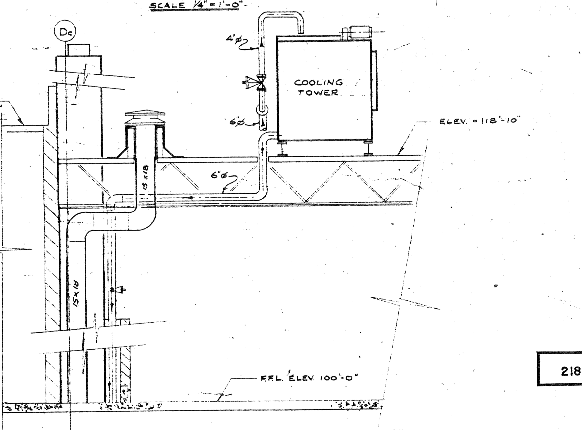
SECTION SHOWING CLEANOUT DOORS FOR EXHAUST CHIMNEY SCALE 1/4\"/>
