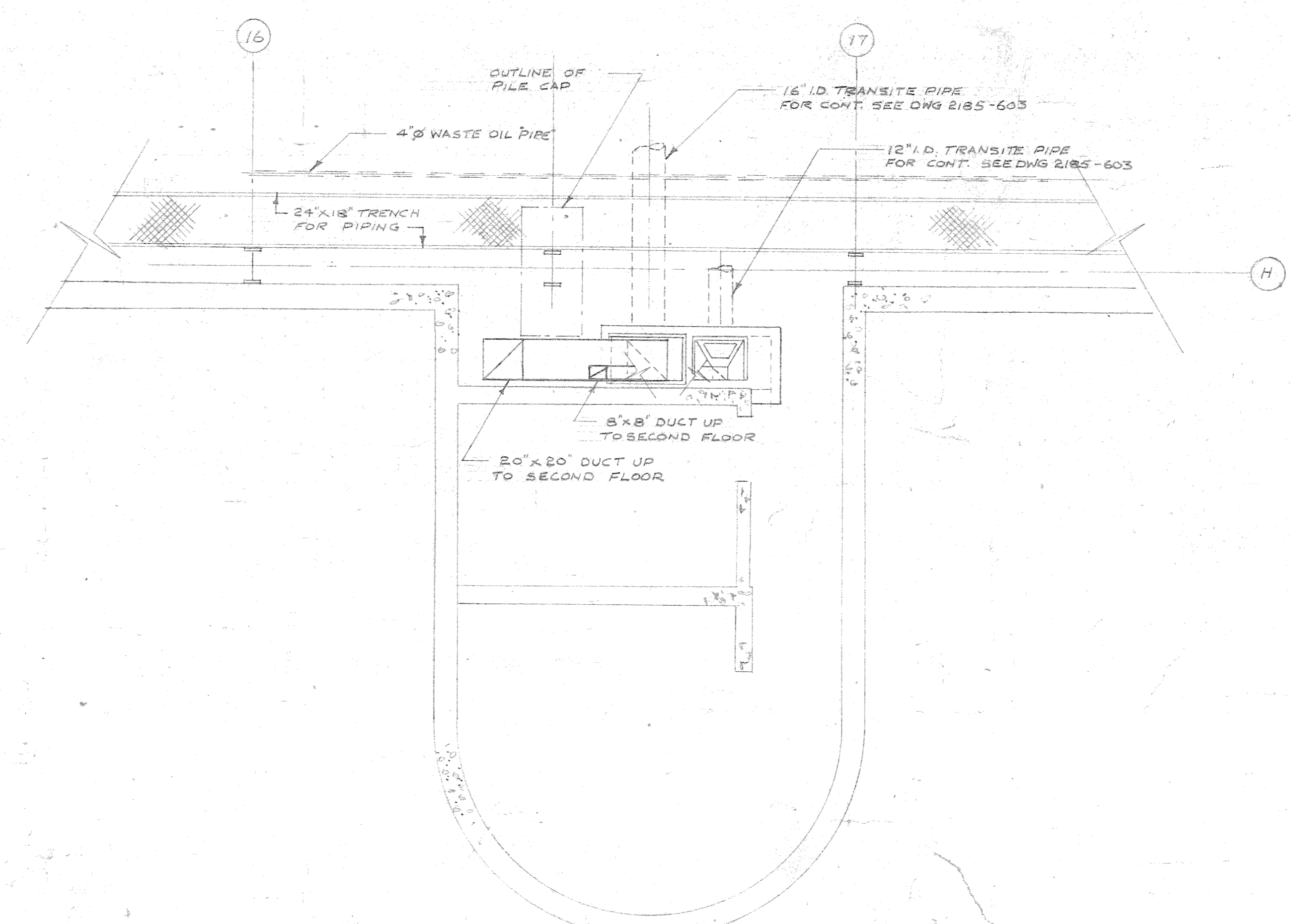
FIRST FLOOR PLAN OF EAST SERVICE PROJECTION OVERHAUL & REPAIR BUILDING SCALE 1/4" = 1'-0"
