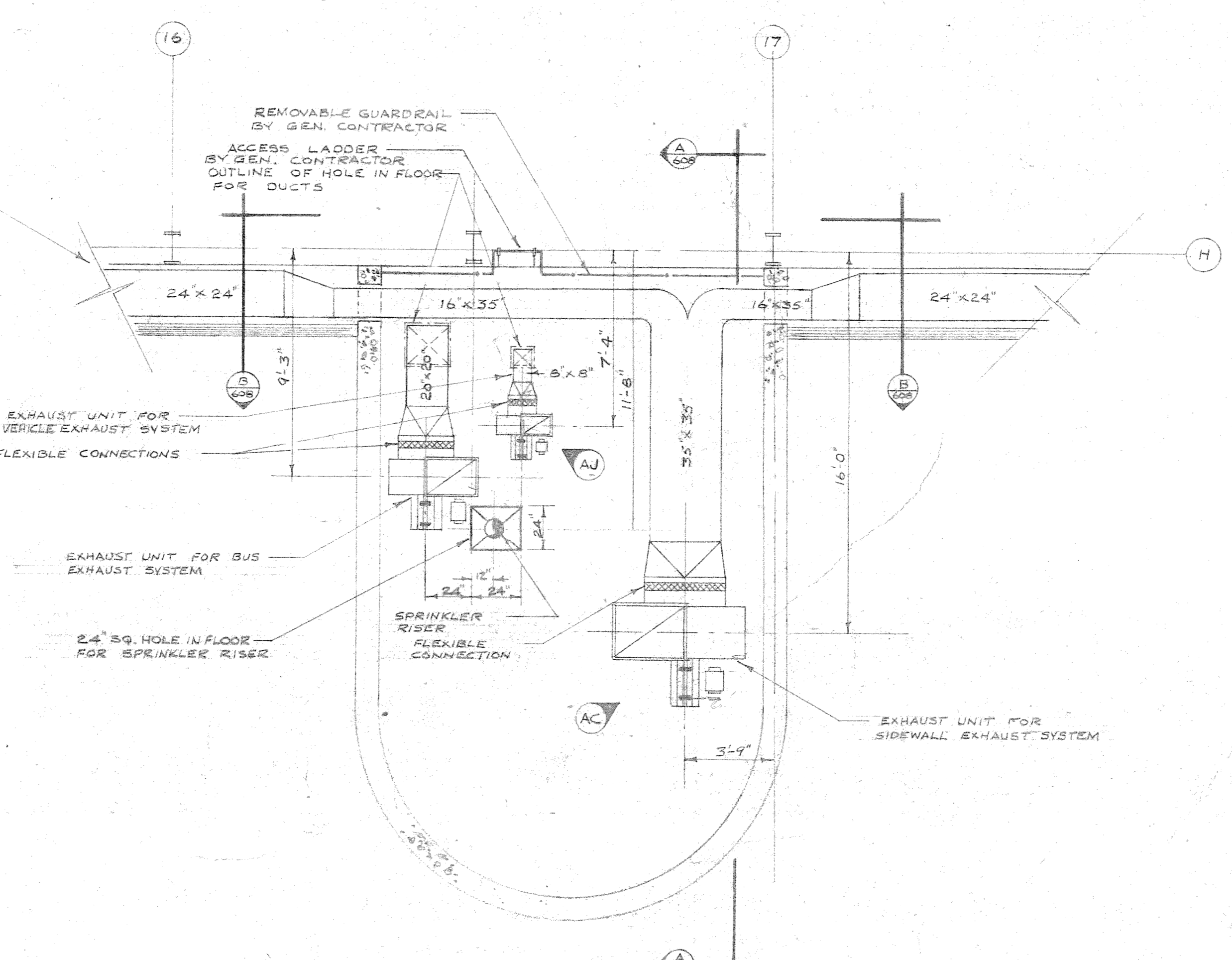
SECOND FLOOR PLAN OF EAST SERVICE PROJECTION OVERHAUL & REPAIR BUILDING SCALE 1/4" = 1'-0"
