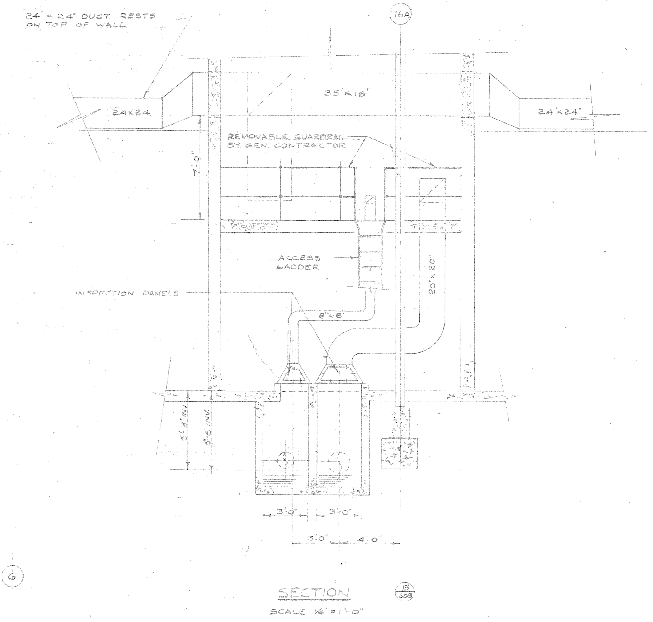
SECTION A-A SCALE 1/4" = 1'-0"
