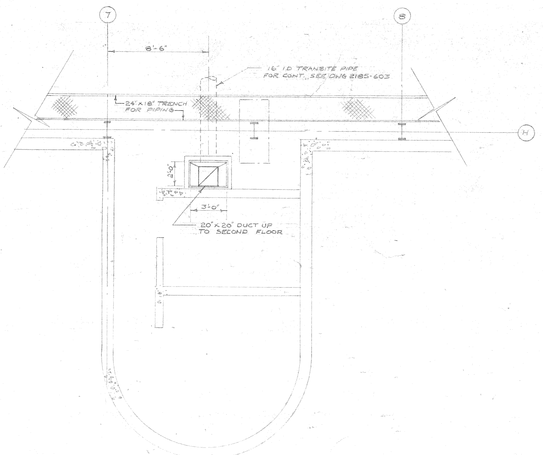
FIRST FLOOR PLAN OF WEST SERVICE PROJECTION OVERHAUL & REPAIR BUILDING SCALE 1/4" = 1'-0"
