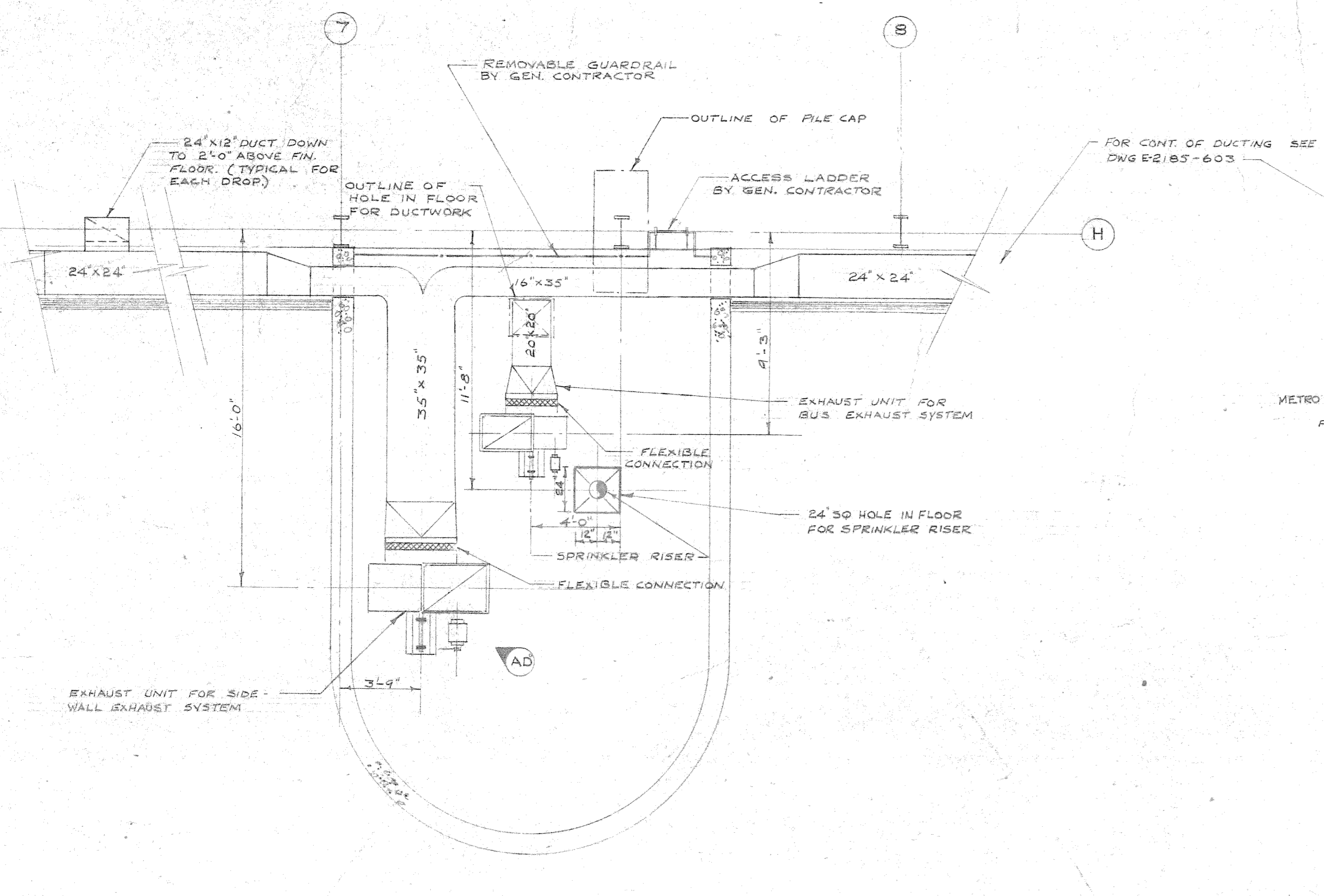
SECOND FLOOR PLAN OF WEST SERVICE PROJECTION OVERHAUL & REPAIR BUILDING SCALE 1/4" = 1'-0"
