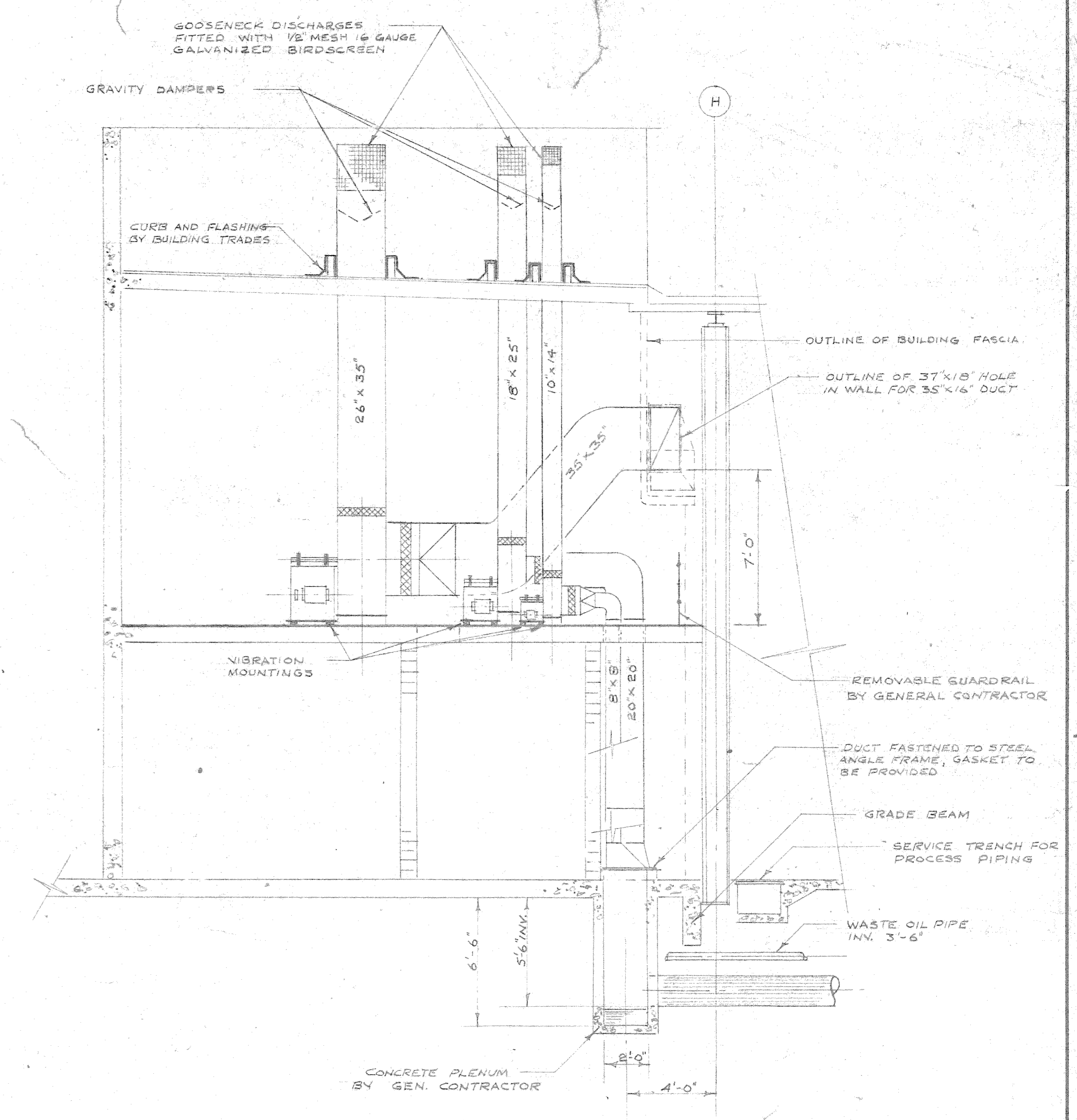
SECTION A-A SCALE 1/4" = 1'-0"
