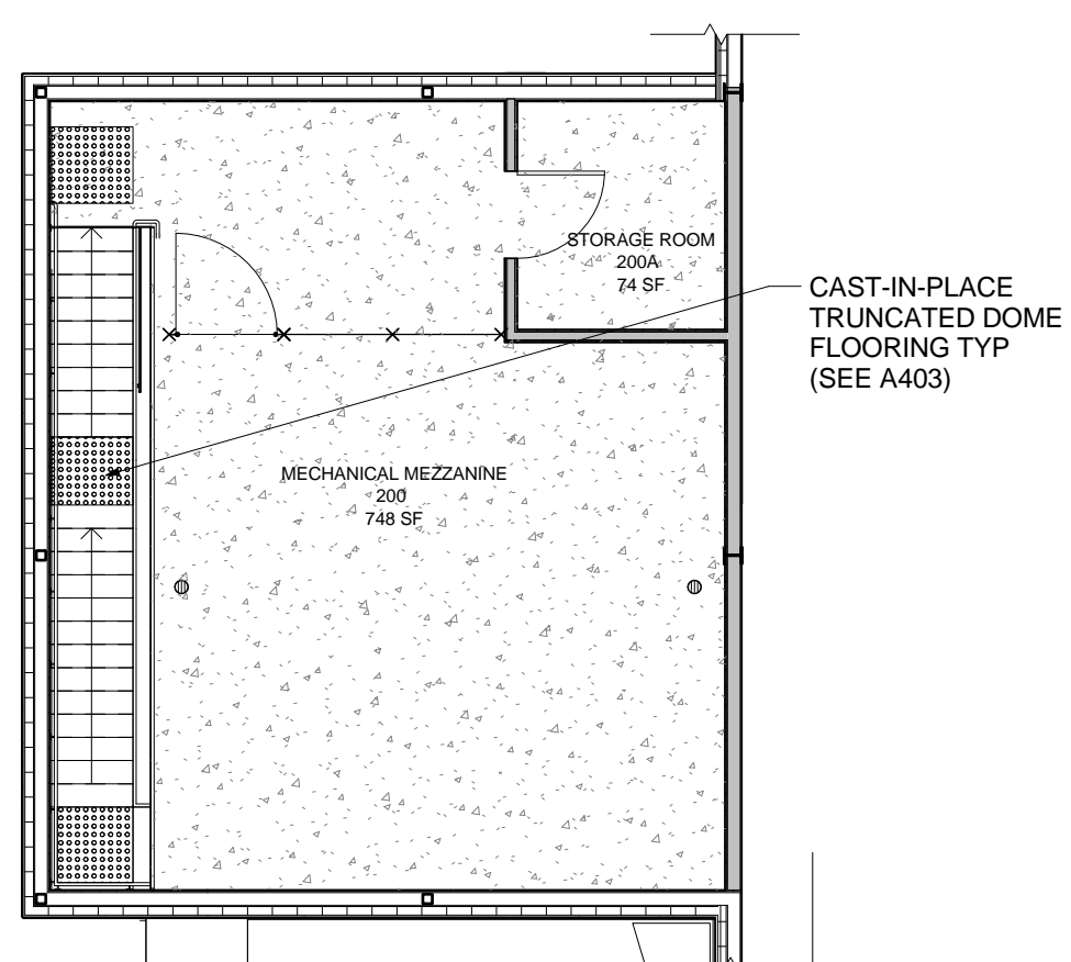
1 FLOORING PLAN - MEZZANINE 1:100
