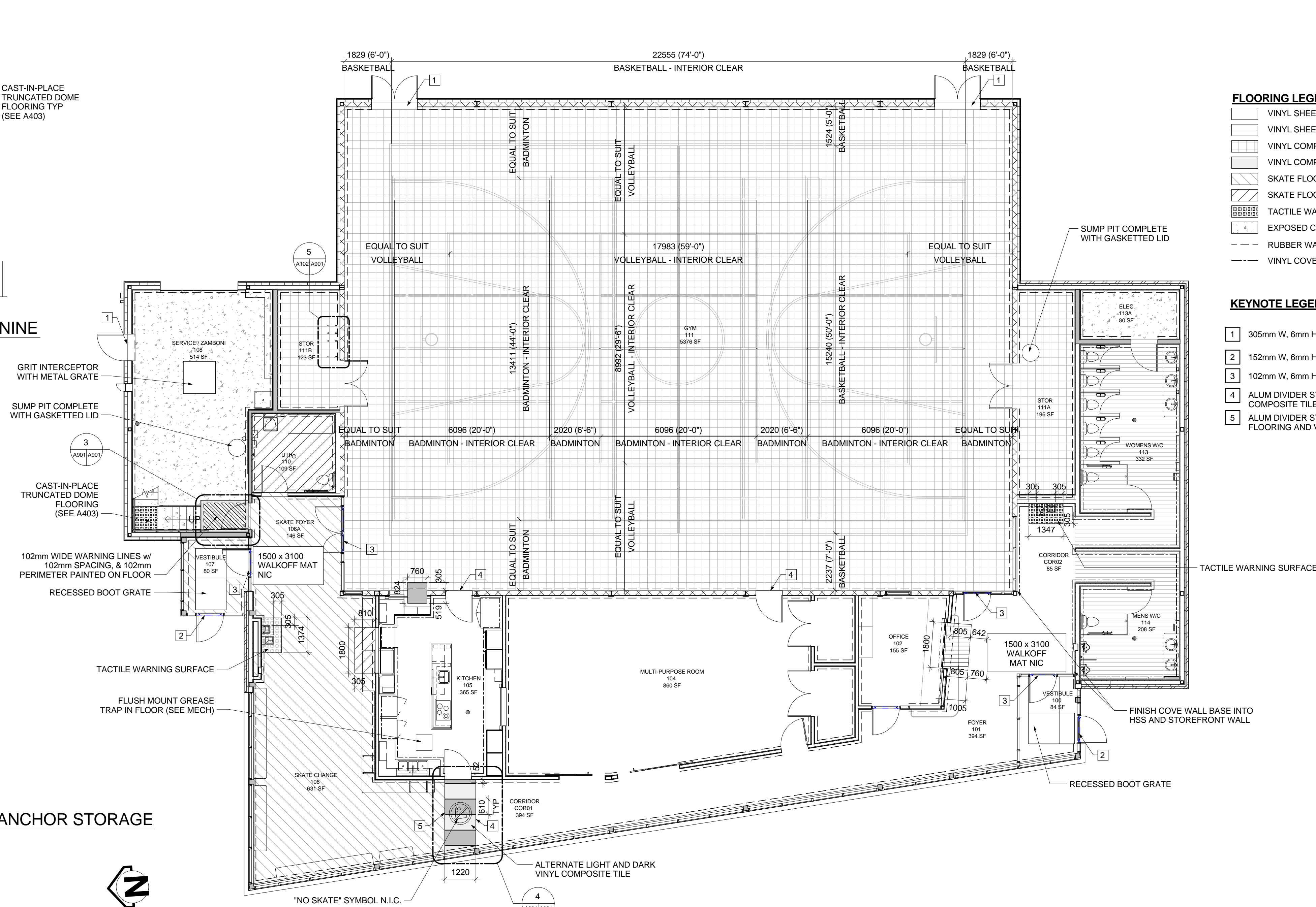
2 FLOORING PLAN - MAIN FLOOR 1:100
