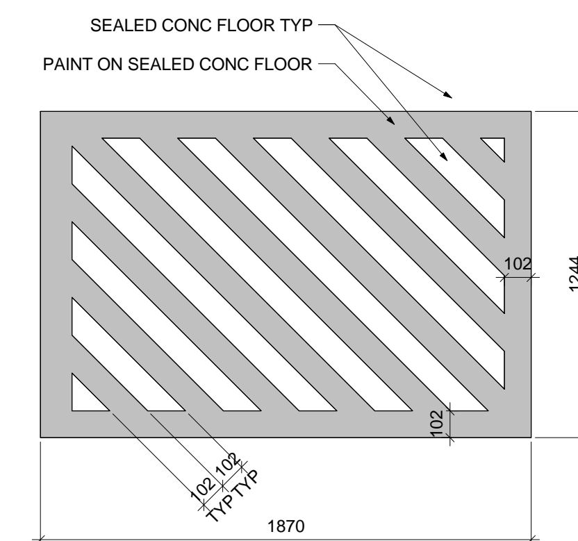
3 FLOOR PAINTING PLAN DETAIL 1:20
