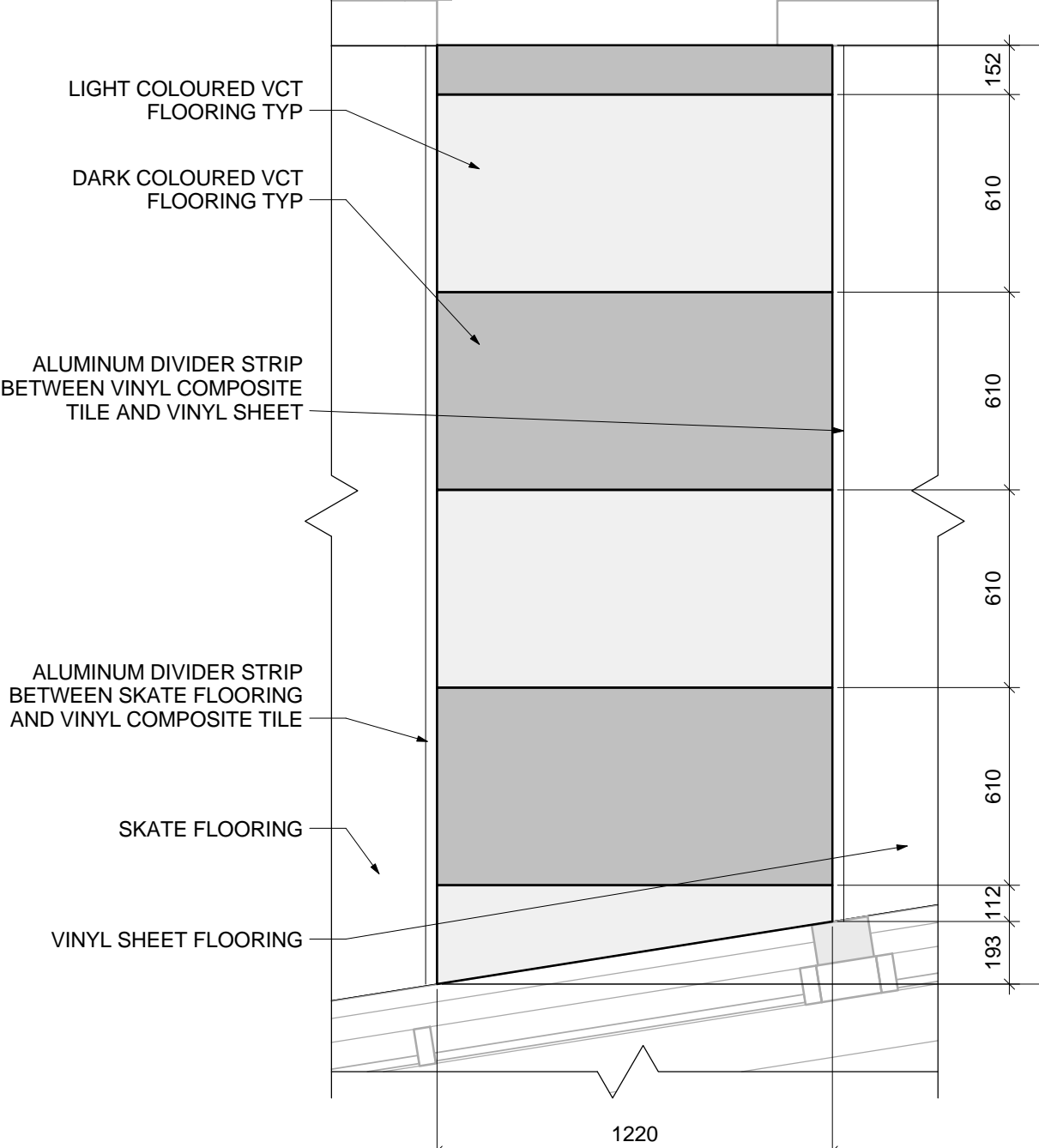
4 FLOOR TRANSITION TILE PATTERN 1:20
