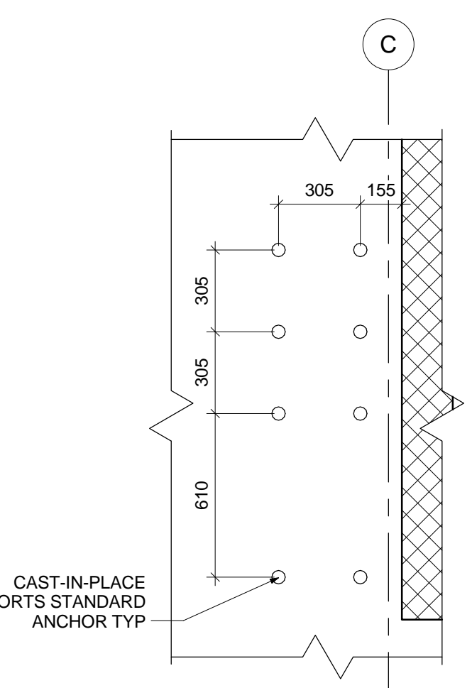
5 CAST-IN-PLACE SPORTS ANCHOR STORAGE 1:20
